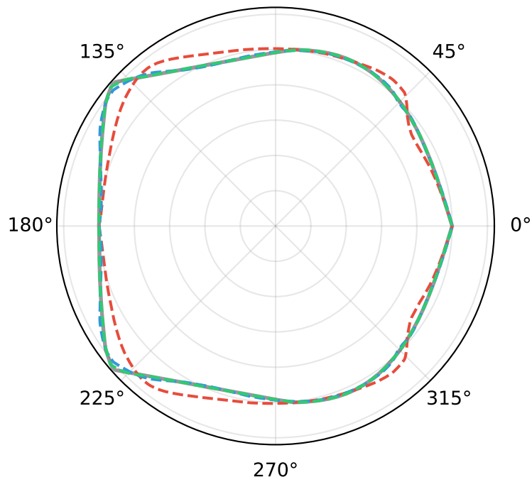
ID: 2 | Sport Fisherman MSE(10): 4.7e-07 90°
