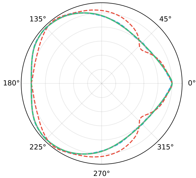
ID: 1 | Sailing yacht MSE(10): 1.9e-07 90° — Truth - - N=3 - · N=10 - · N=40
