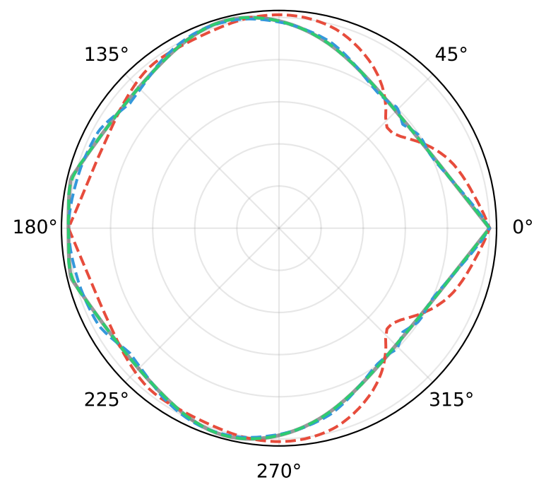
ID: 64 | Sparkman & Step MSE(10): 6.9e-07 90°
