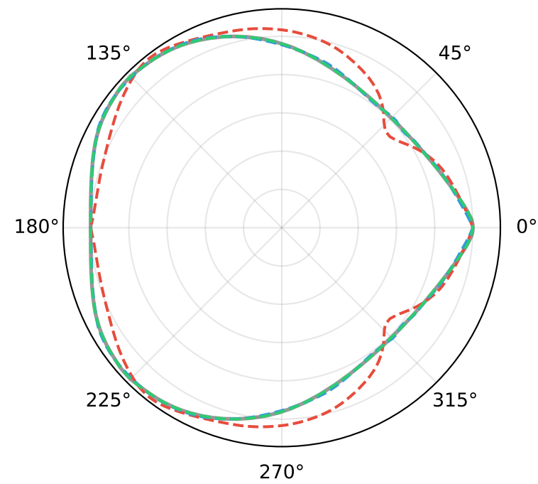
ID: 237 | 40 sailing yach MSE(10): 1.9e-07 90°
