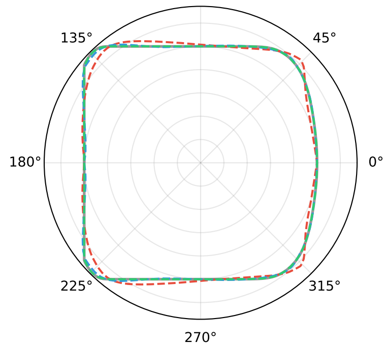
ID: 241 | 120m containers MSE(10): 1.8e-07 90°
