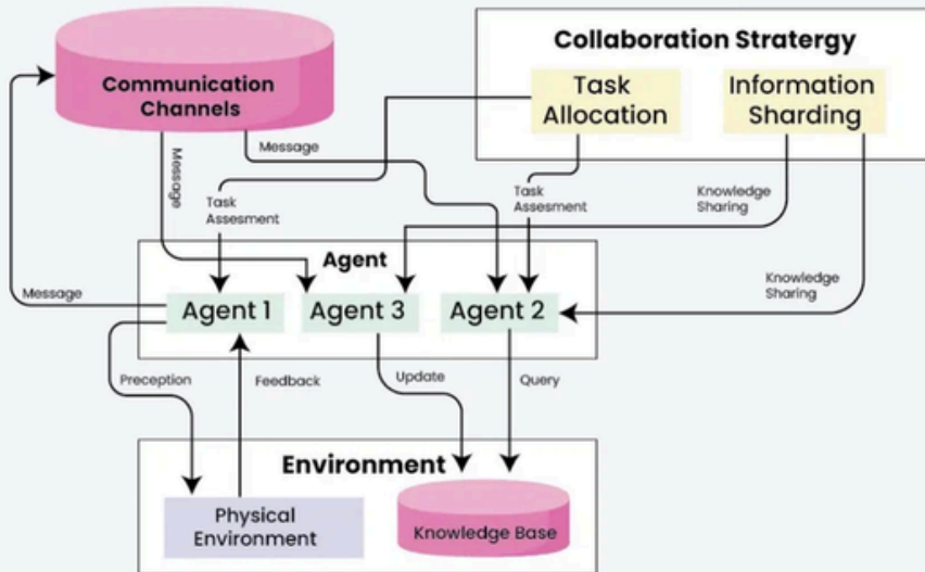
Multiagent system Architecture
