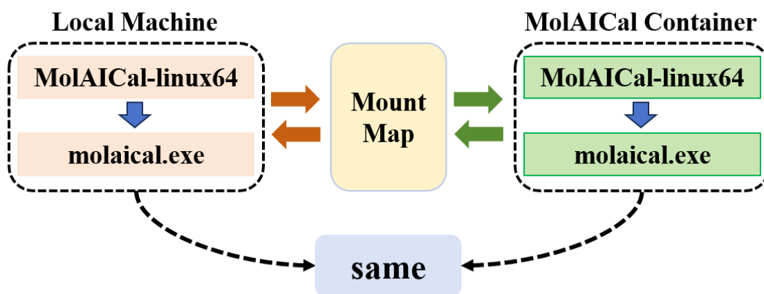
Figure 3.2.5.1 Architecture Diagram for the Linux Version of MolAICal
