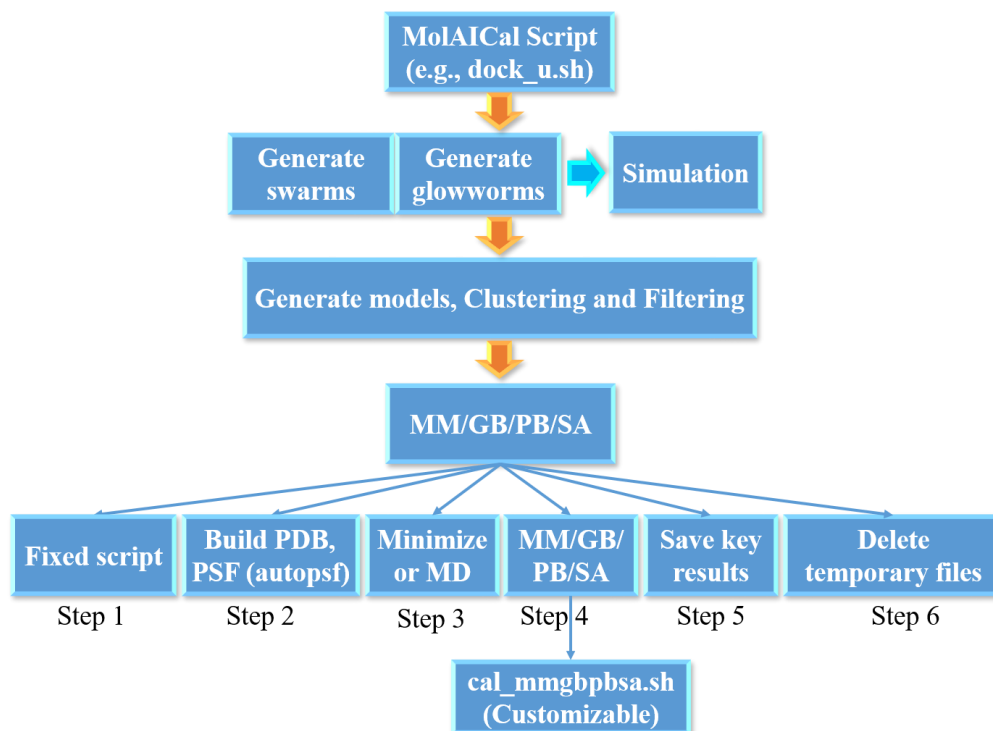
Part I Figure 6.2.4.2 Docking unit.
