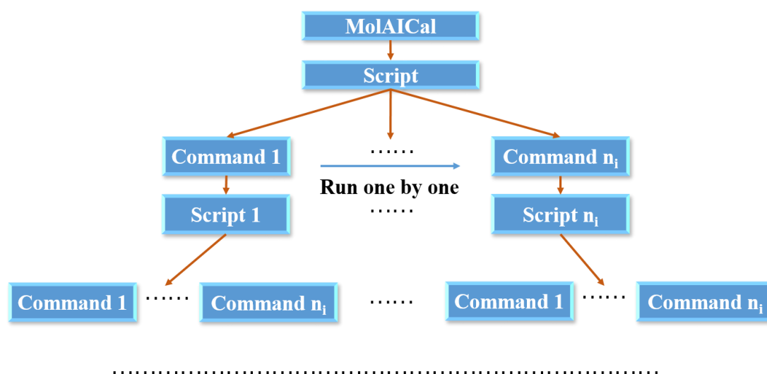
Part I Figure 6.2.8 The framework of MolAICal script
