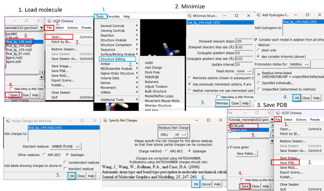
Figure 1. Minimize molecule
