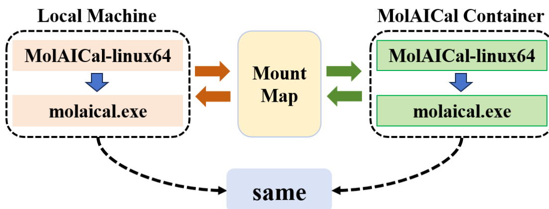
Figure 10. Architecture Diagram for the Linux Version of MolAICal
