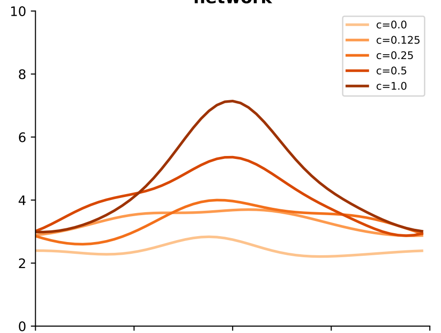
network
