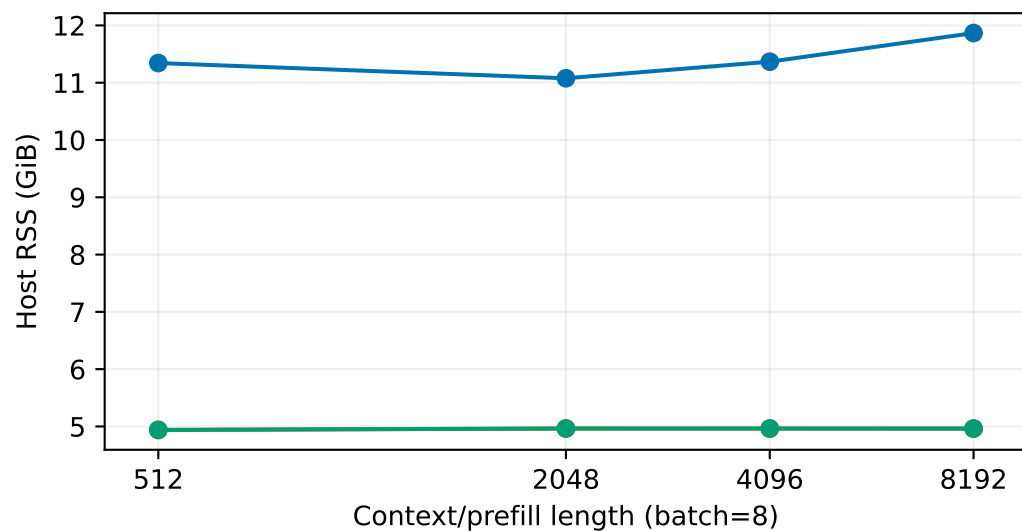
decode
