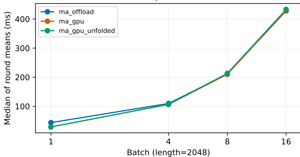
decode
