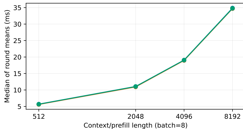
decode
