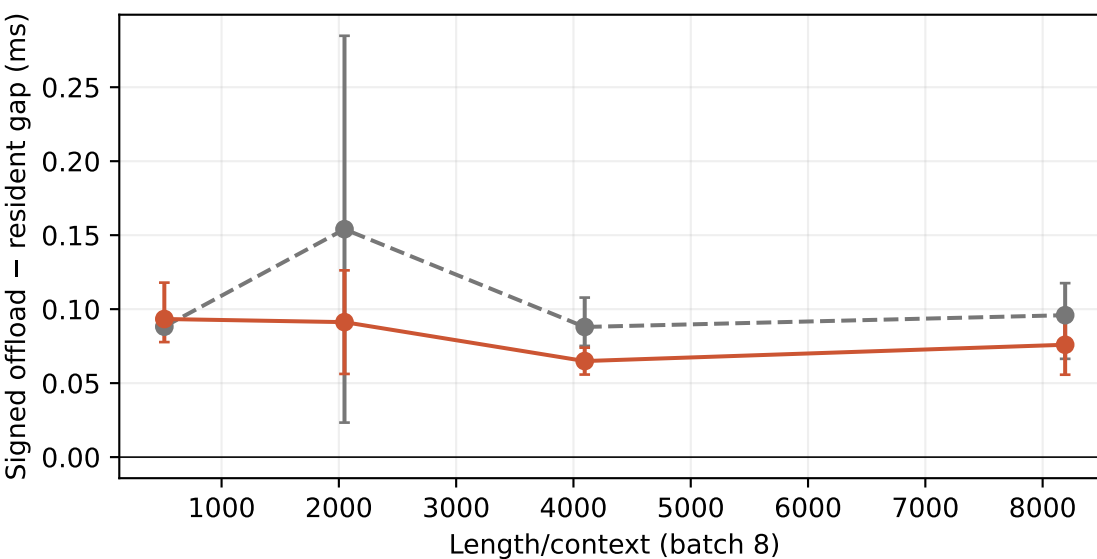
Decode
