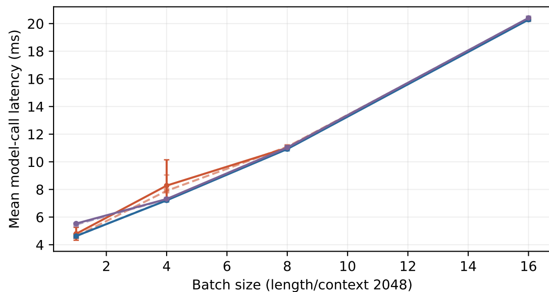
Decode
