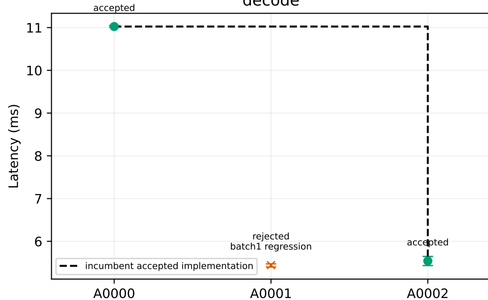
decode
