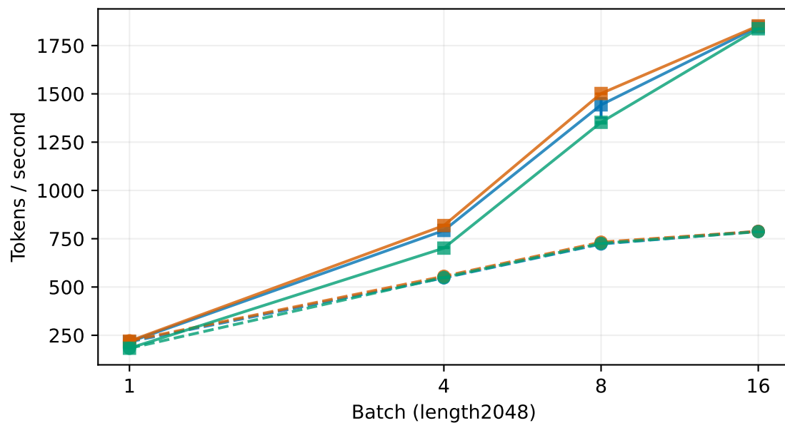
decode
