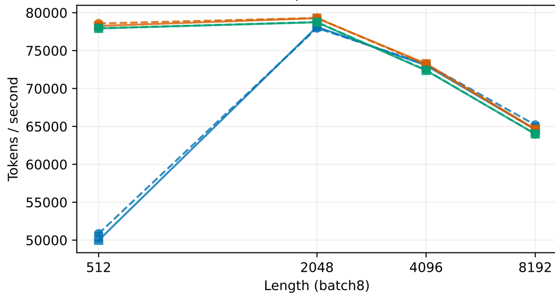
decode
