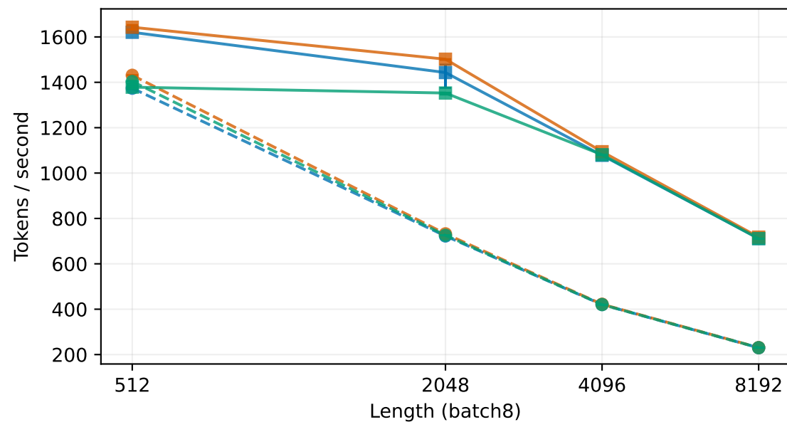
decode
