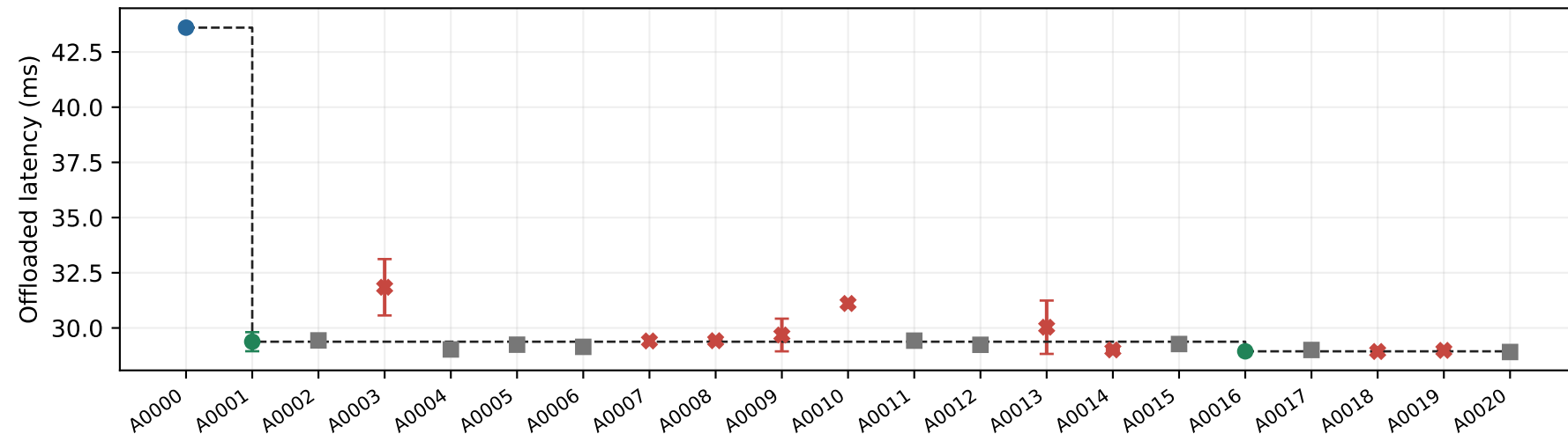
Prefill, batch 8, length/context 2048
