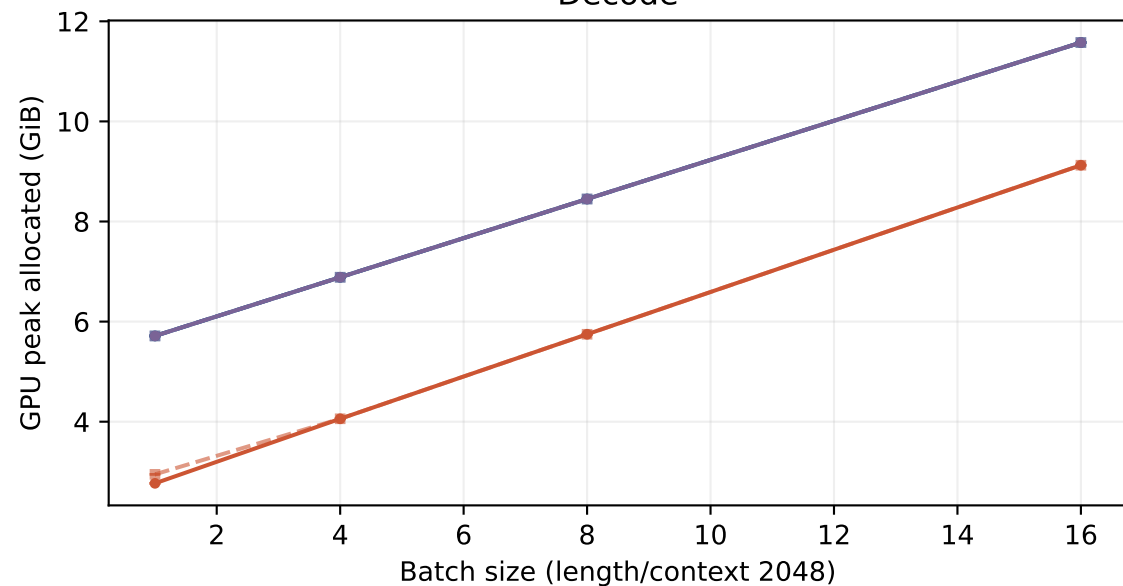
Decode
