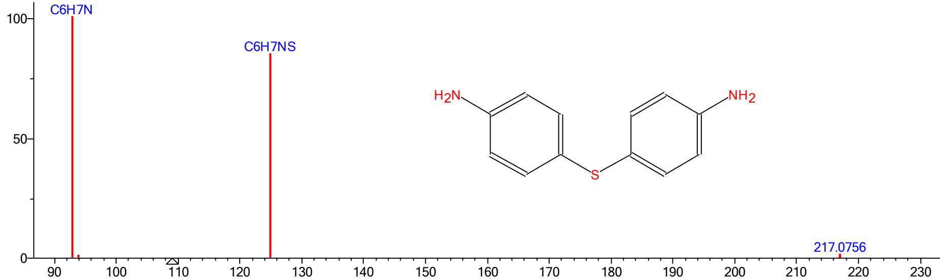
(hr_msms_nist) 4,4'-Thiodianiline [M+2H] 2+ IT-FT 35% P=109
