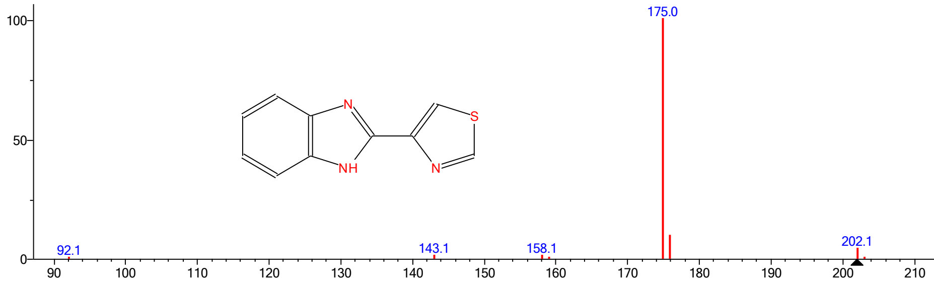
(lr_msms_nist) Thiabendazole [M+H] + IT 35% P=202
