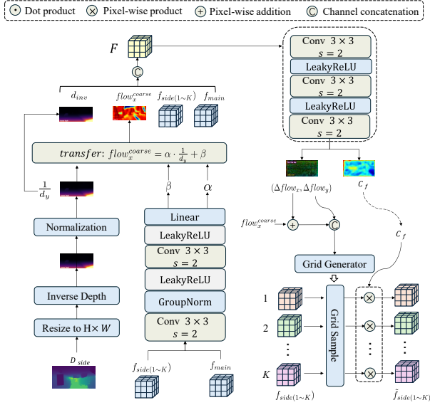
Fig. 4: Depth-Aware Geometric Alignment (DAGA). It predicts global affine parameters (\alpha, \beta) to construct a depth-guided coarse flow, refines it with a residual flow, and warps the K side features. A learned confidence mask c_f is used to suppress unreliable regions.
