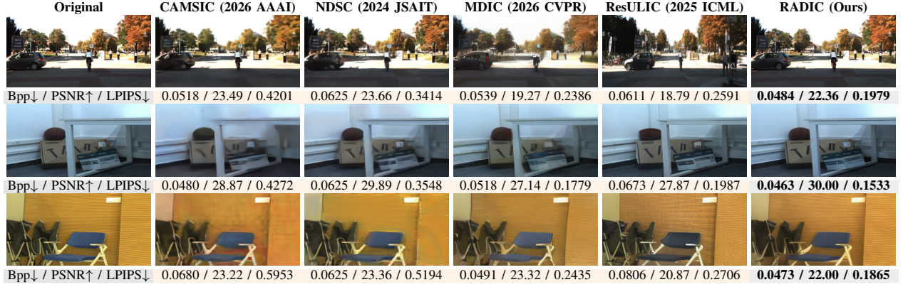
Fig. 7: Qualitative comparison among CAMSIC [16], NDSC [6], MDIC [7], ResULIC [24], and RADIC. CAMSIC and NDSC exhibit severe degradation at extremely low bitrates, while RADIC has the lowest LPIPS in the displayed examples. PSNR varies by image and method.
