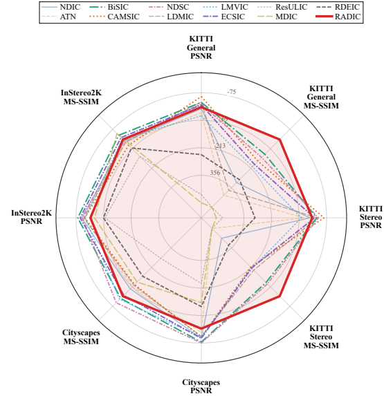
Fig. 6: Comparison of BD-Rate (%) [40], [41] computed with PSNR and MS-SSIM as quality metrics on four test datasets. RADIC is used as the anchor, and lower BD-Rate indicates better rate-distortion performance.
