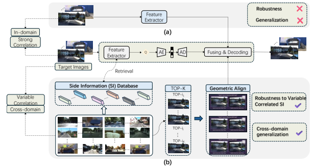
Fig. 1: Comparison of two DIC settings. (a) Existing methods [6], [7] rely on a paired SI for each target. (b) The proposed RADIC retrieves top- K references from a decoder-only visual database, aligns them geometrically, and uses the aligned features for reconstruction, thereby relaxing the paired-SI assumption.
