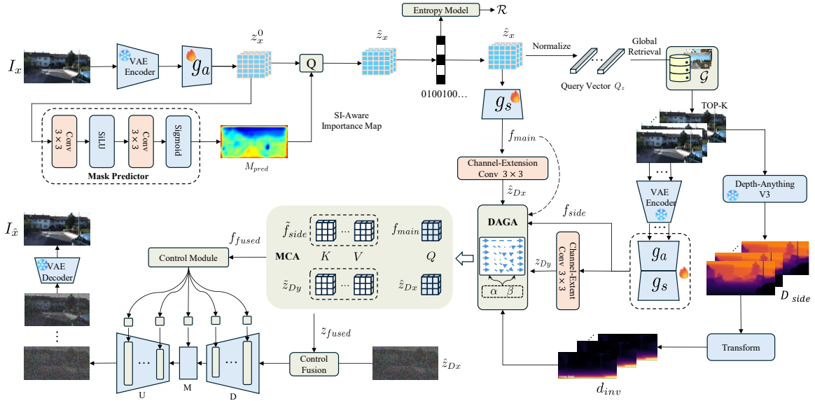
Fig. 3: Overall architecture of RADIC. The encoder maps the target image I_x to a latent representation z_x and predicts an SI-aware importance map M_{\text{pred}} for latent modulation before quantization. At the decoder, \hat{z}_x retrieves top- K references from the gallery \mathcal{G} , which are aligned by Depth-Aware Geometric Alignment (DAGA) and screened by Multi-reference Cross-Attention (MCA). The fused reference features condition a latent diffusion model to reconstruct \hat{I}_x at extremely low bitrates.
