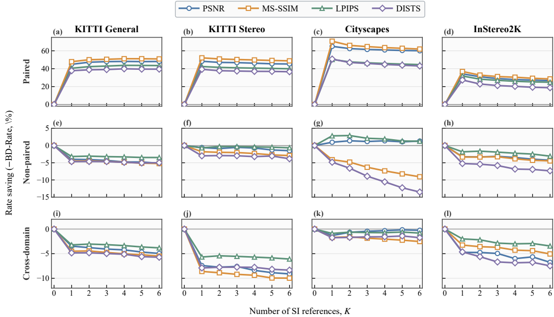
Fig. 8: Effect of the number of SI references under paired, non-paired, and cross-domain SI. Rate saving is defined as the negative BD-Rate relative to K = 0 under the same SI setting, where higher values indicate better coding efficiency.
