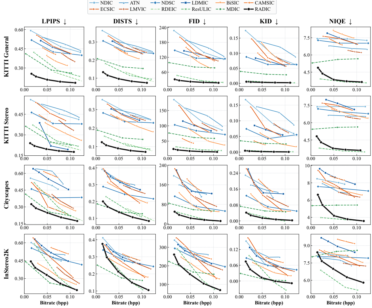
Fig. 5: Rate-perception comparisons on four test datasets. Lower ( \downarrow ) is better for all metrics.
