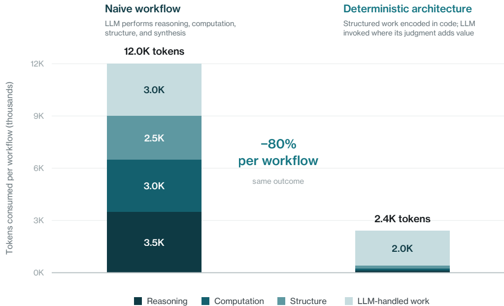
Figure 5. Cost per workflow: naive versus deterministic architecture. The same business outcome can be produced with substantially lower token consumption when structured work is encoded in deterministic code and the LLM is invoked where it adds value. Illustrative; reductions in production deployments vary by workflow complexity, and the architecture is best applied where workflows have stable, repeatable structure.
