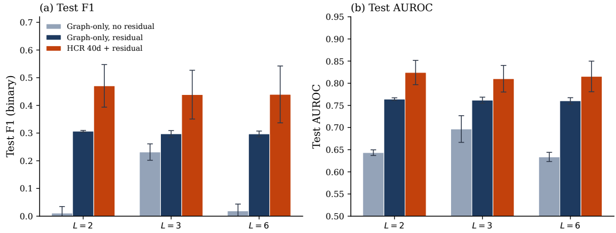
Figure 8.3: IEEE-CIS-G ablation of residual connections and the statistical evidence branch.
