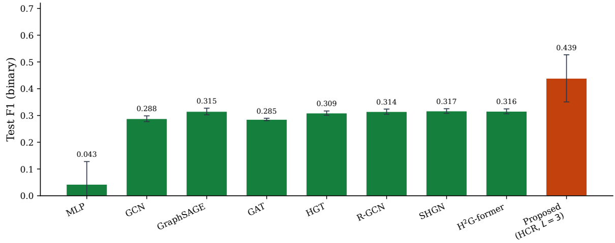
Figure 8.4: IEEE-CIS-G test F1 against selected H2GB baselines from Table 3 of [28]
