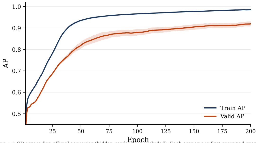
Full model — train vs validation AP
