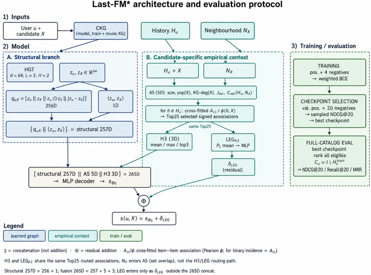
Figure 6.2: Last-FM* architecture. Structural HGT yields [q_{uX} \parallel \langle z_u, z_X \rangle] \in \mathbb{R}^{257} . A5 uses H_u , X and N_X ; routed Top25 associations feed both H3 and \text{LEG}_{K2} , with LEG entering only as residual \delta_{\text{LEG}} . Late fusion is 265-dimensional ( \parallel = concatenation; \oplus = residual addition). The right column summarizes training and the two development evaluation levels; the sealed external benchmark is defined in Section 6.4.
