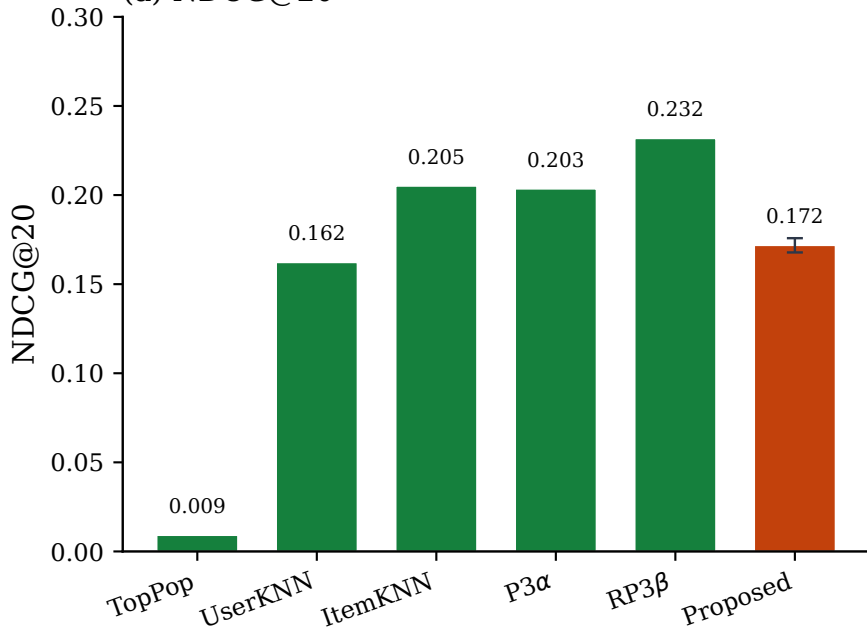
(a) NDCG@20
