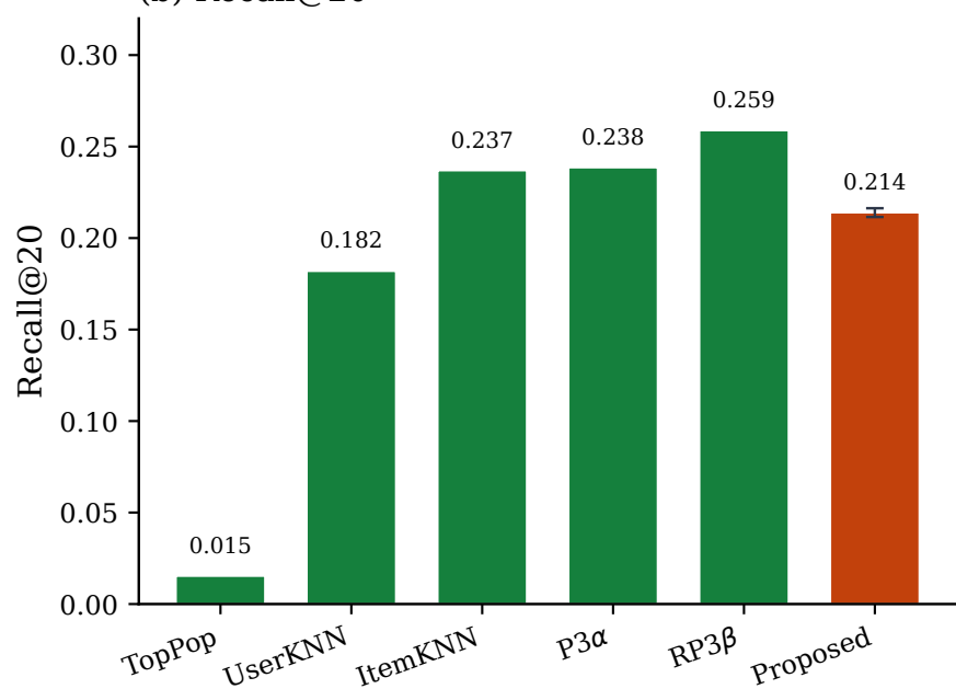
(b) Recall@20
