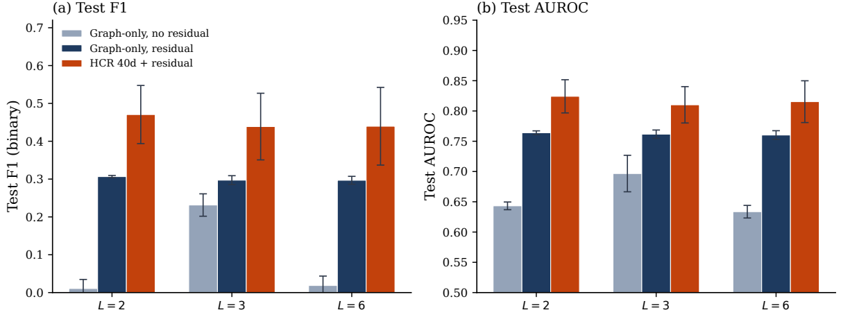
Figure 8.3: IEEE-CIS-G ablation of residual connections and the statistical evidence branch.
