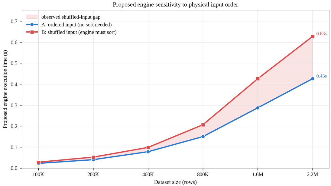
Figure 6-14: Engine time on ordered vs shuffled input, across sizes.
