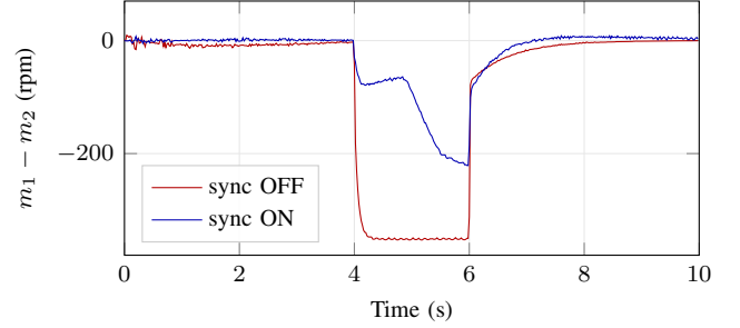
Fig. 8: Single-track load disturbance ( 1.0\text{ N m} on Motor 1, t = 4\text{--}6 s): inter-motor speed difference, synchronization ON vs OFF. The loaded motor saturates; synchronization slows the other motor to match, cutting the sustained difference from \sim 344 to \sim 125 rpm.
