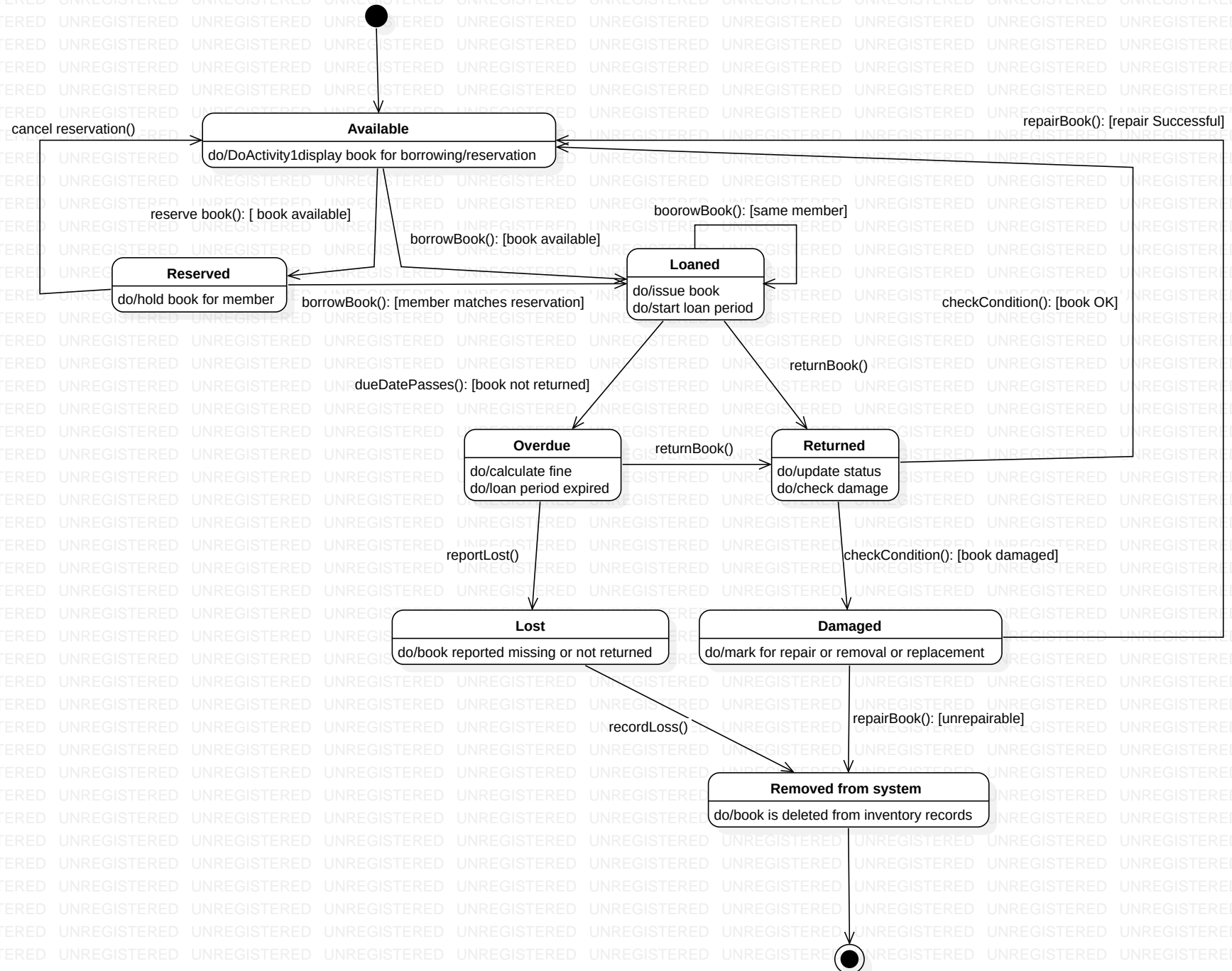
StateMachine1::StatechartDiagram1
