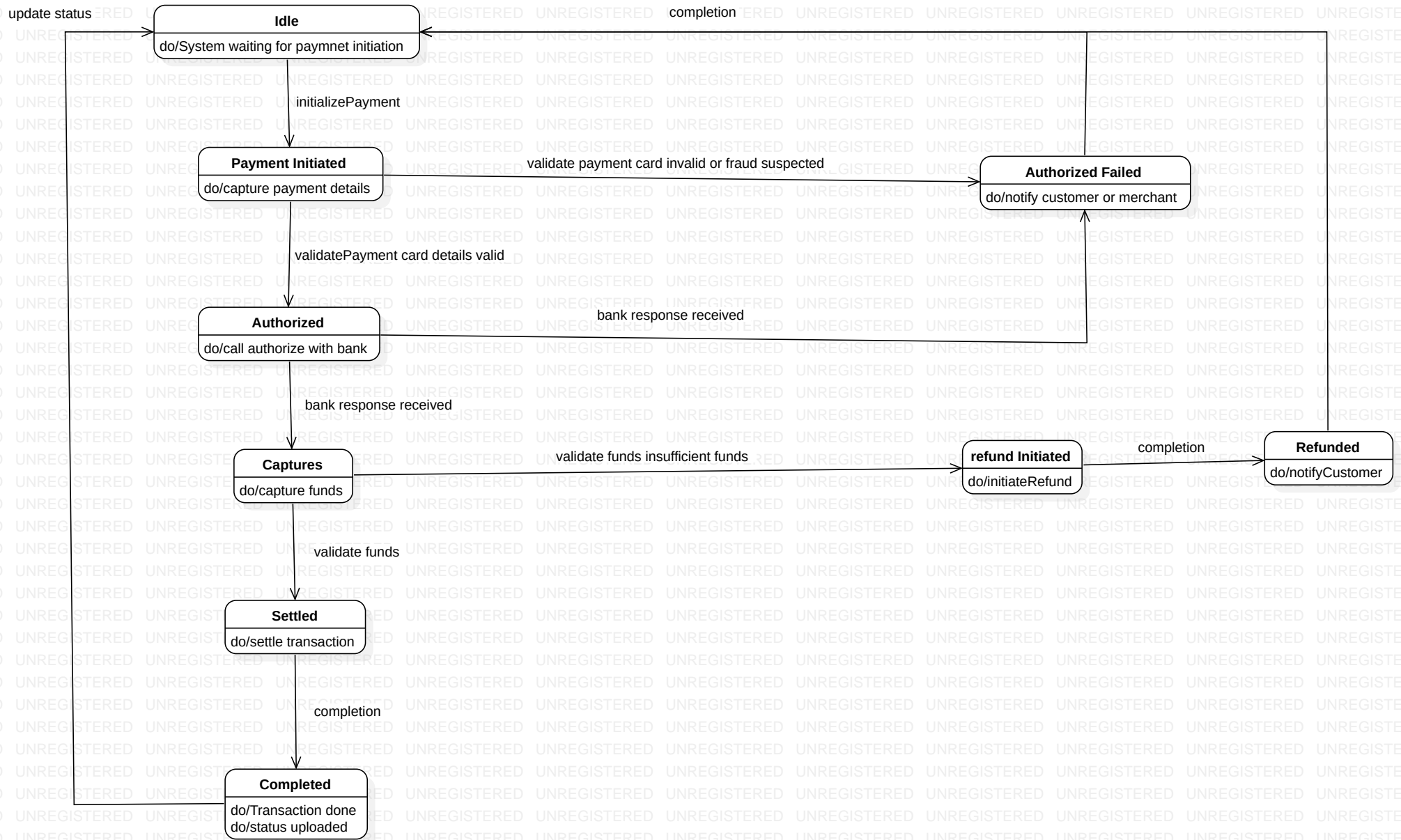
StateMachine1::StatechartDiagram1
