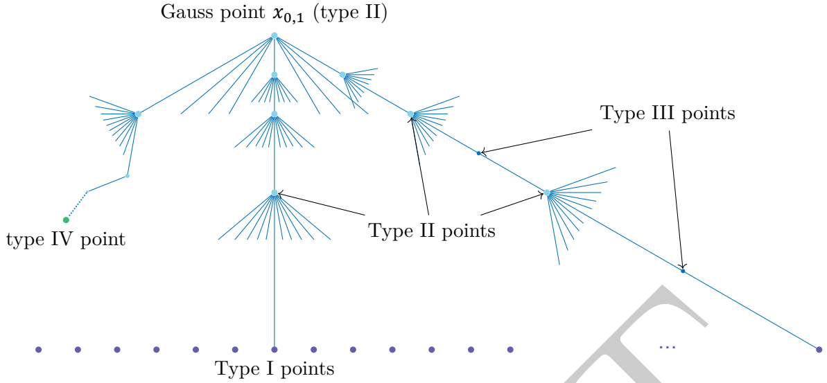
Figure 4.1: The Berkovich spectrum \mathcal{M}(\mathbb{k}\{T\})
