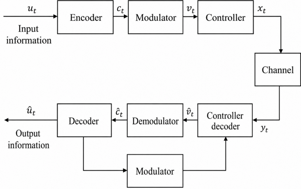
Figure 1.1: Block diagram of the BIBCM-ID system model redrawn from the reference thesis structure.
