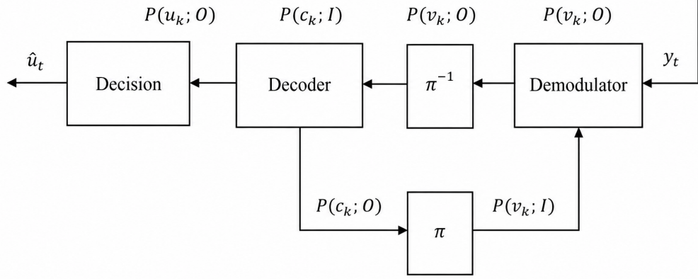
Figure 1.2: Soft-information exchange in the iterative BIBCM-ID receiver redrawn in English.
