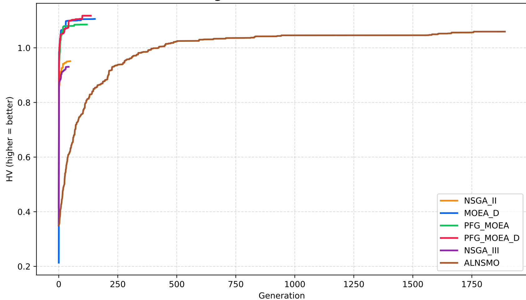
HV Convergence - data100 - C - h100c106
