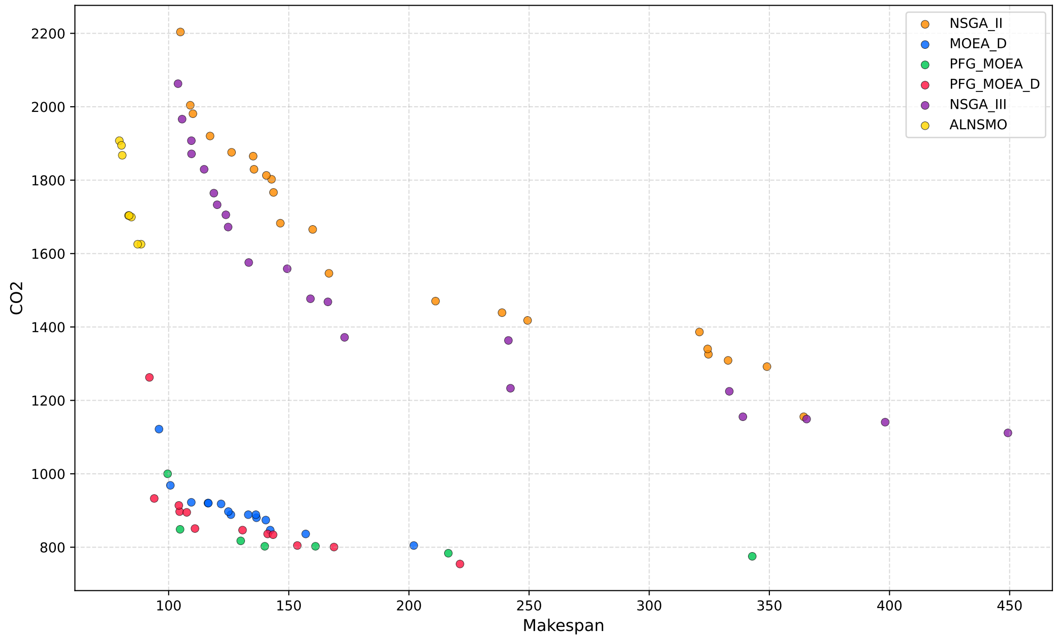
Pareto Front - data100 - R - h100r208
