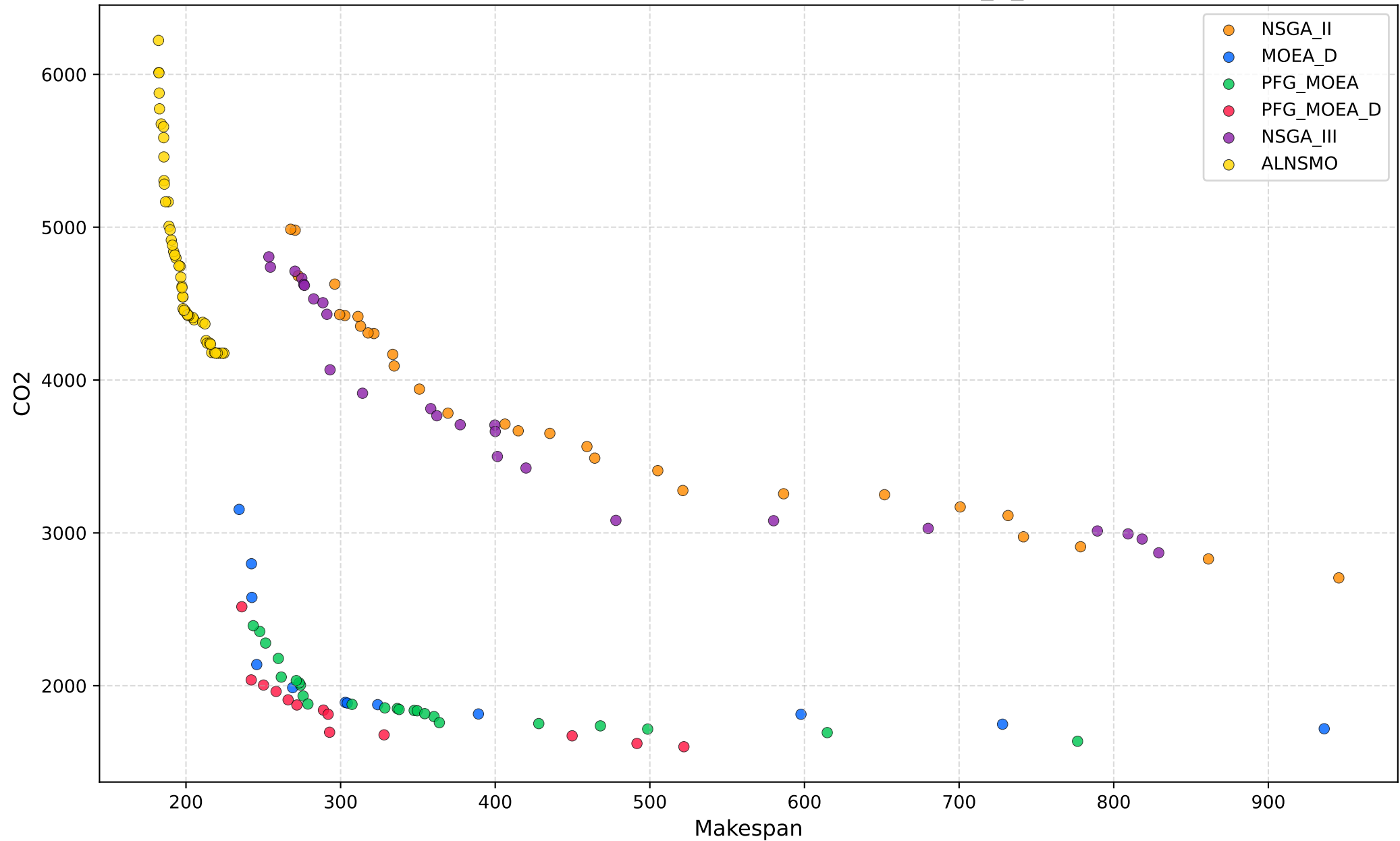
Pareto Front - data200 - RC - h200RC1_2_10
