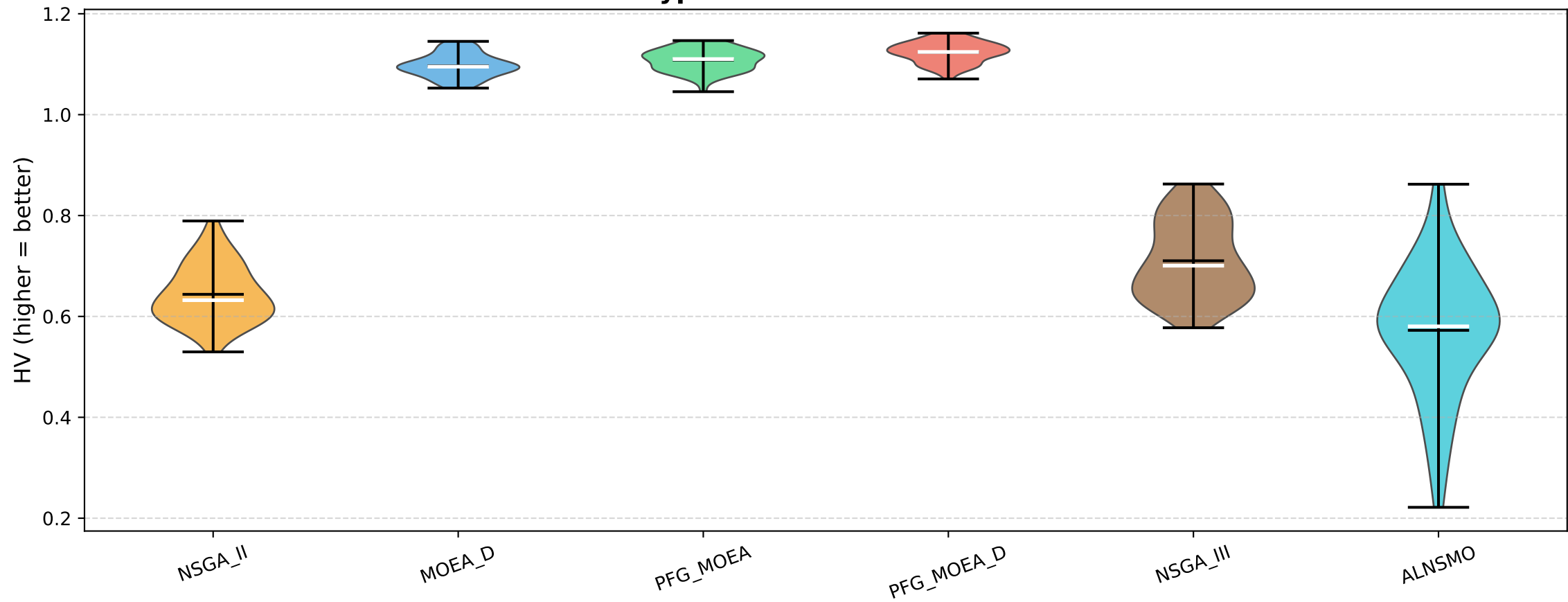
Hypervolume Distribution
