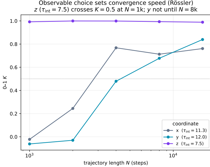
FIG. 6. Observable selection for the Rössler system: the 0–1 K versus trajectory length for each state coordinate. The z coordinate ( \tau_{\text{int}} = 7.5 ) is already converged ( K \approx 1 ) at N = 1,000 steps, whereas y ( \tau_{\text{int}} = 12 ) does not cross K = 0.5 until N = 8,000 . Shorter integrated autocorrelation time gives faster convergence.
