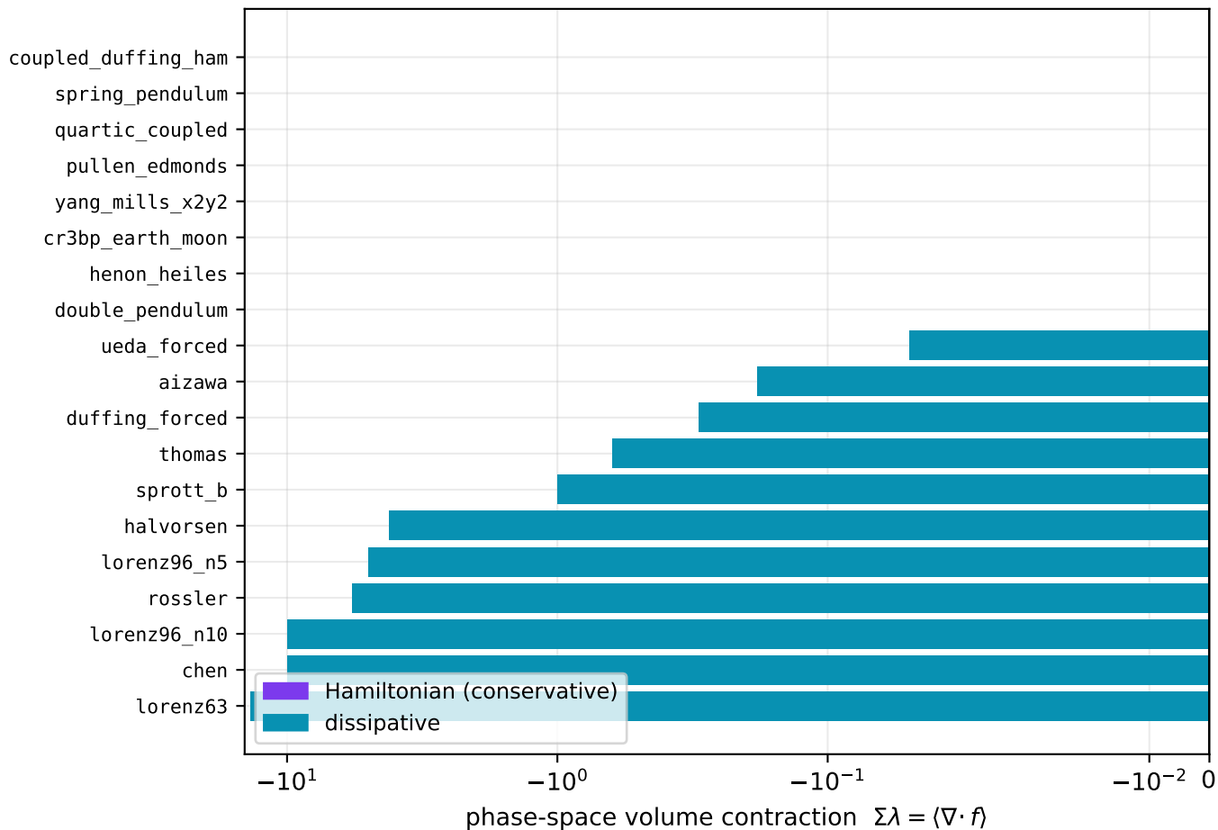
The discriminator: \Sigma\lambda = 0 (Hamiltonian) vs < 0 (dissipative)
