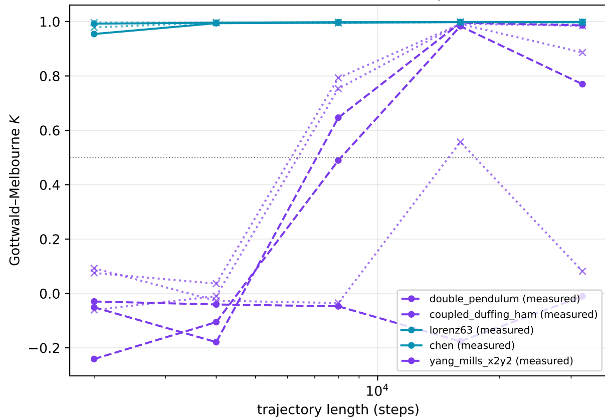
0-1 K is length-dependent for Hamiltonian flows (dotted = closed-form Green-Kubo prediction)
