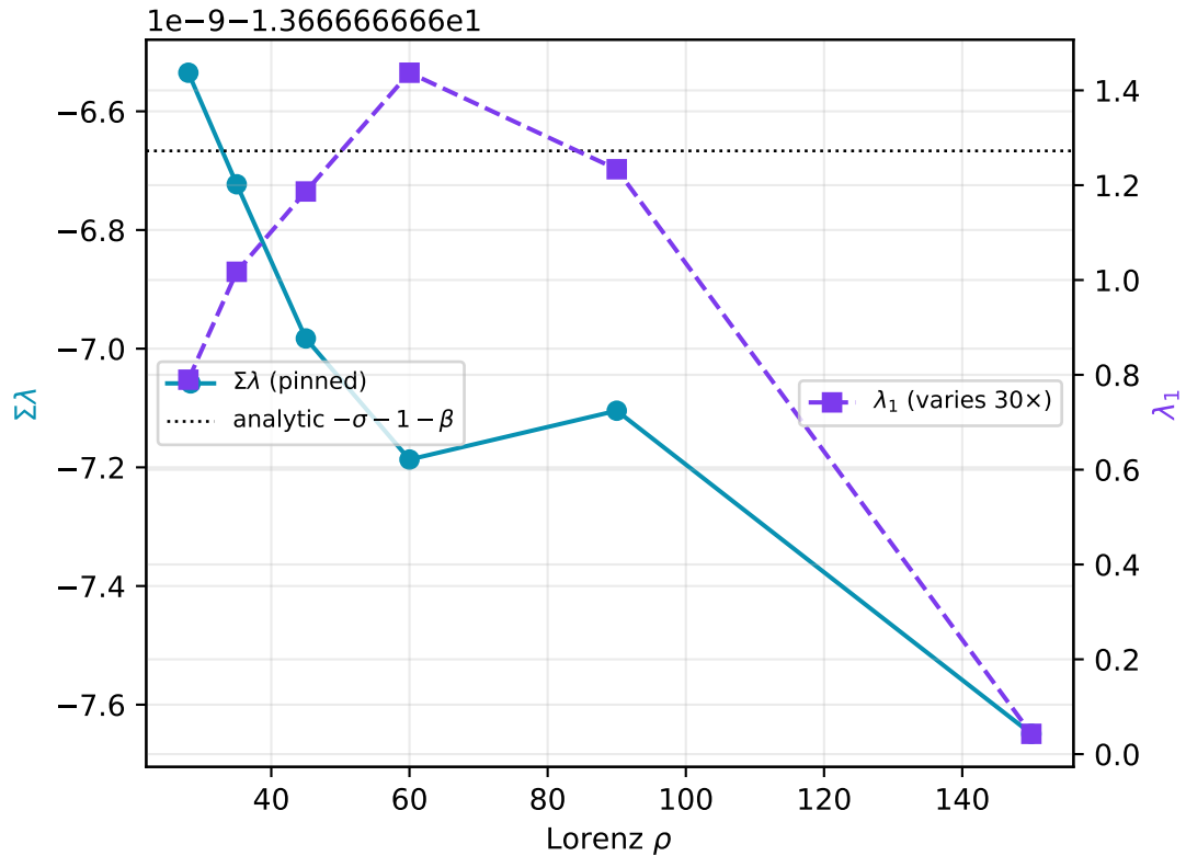
\Sigma\lambda is chaos-strength-independent
