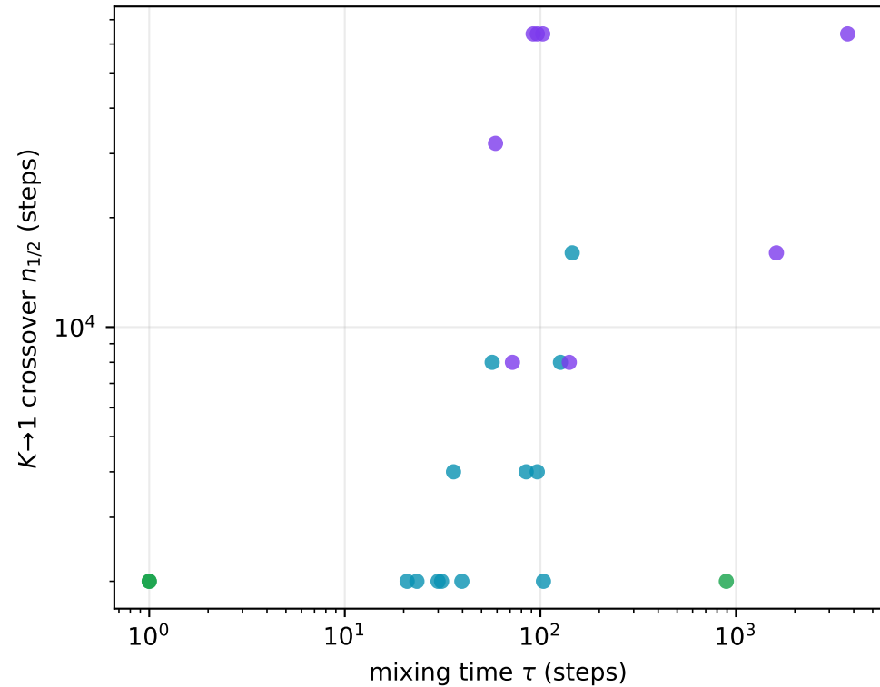
Mixing-time law (Spearman \rho = 0.58 )
