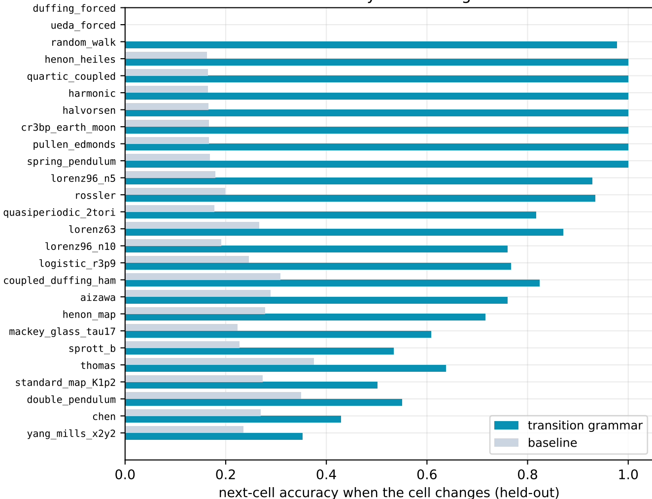
Predict the climate: itinerary transition grammar vs baseline
