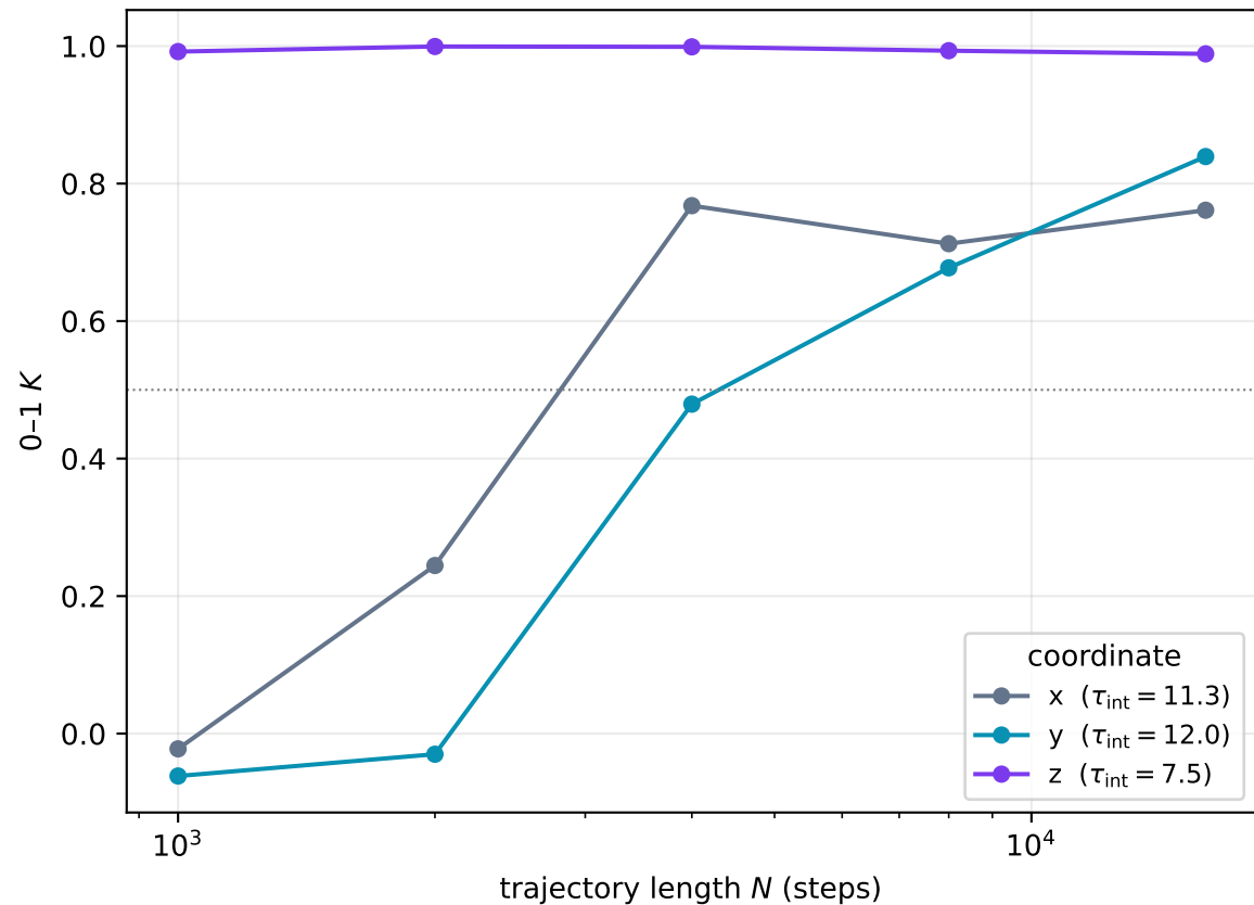
Observable choice sets convergence speed (Rössler) z ( \tau_{\text{int}} = 7.5 ) crosses K = 0.5 at N = 1\text{k} ; y not until N = 8\text{k}
