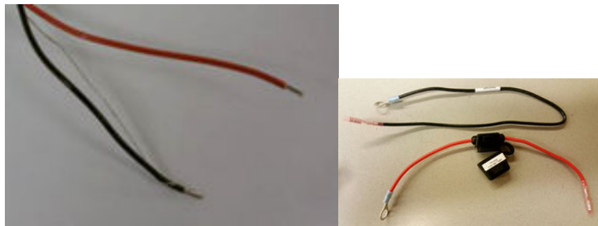
Figure 48: Black and Silver Drain Wires Twisted and Cramped
