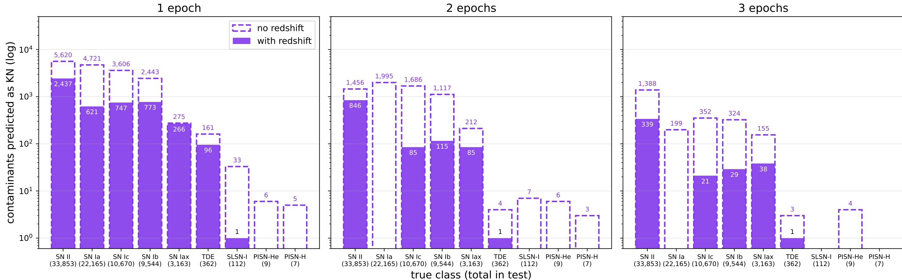
Contaminants leaking as KN by true class (threshold=0.2)
