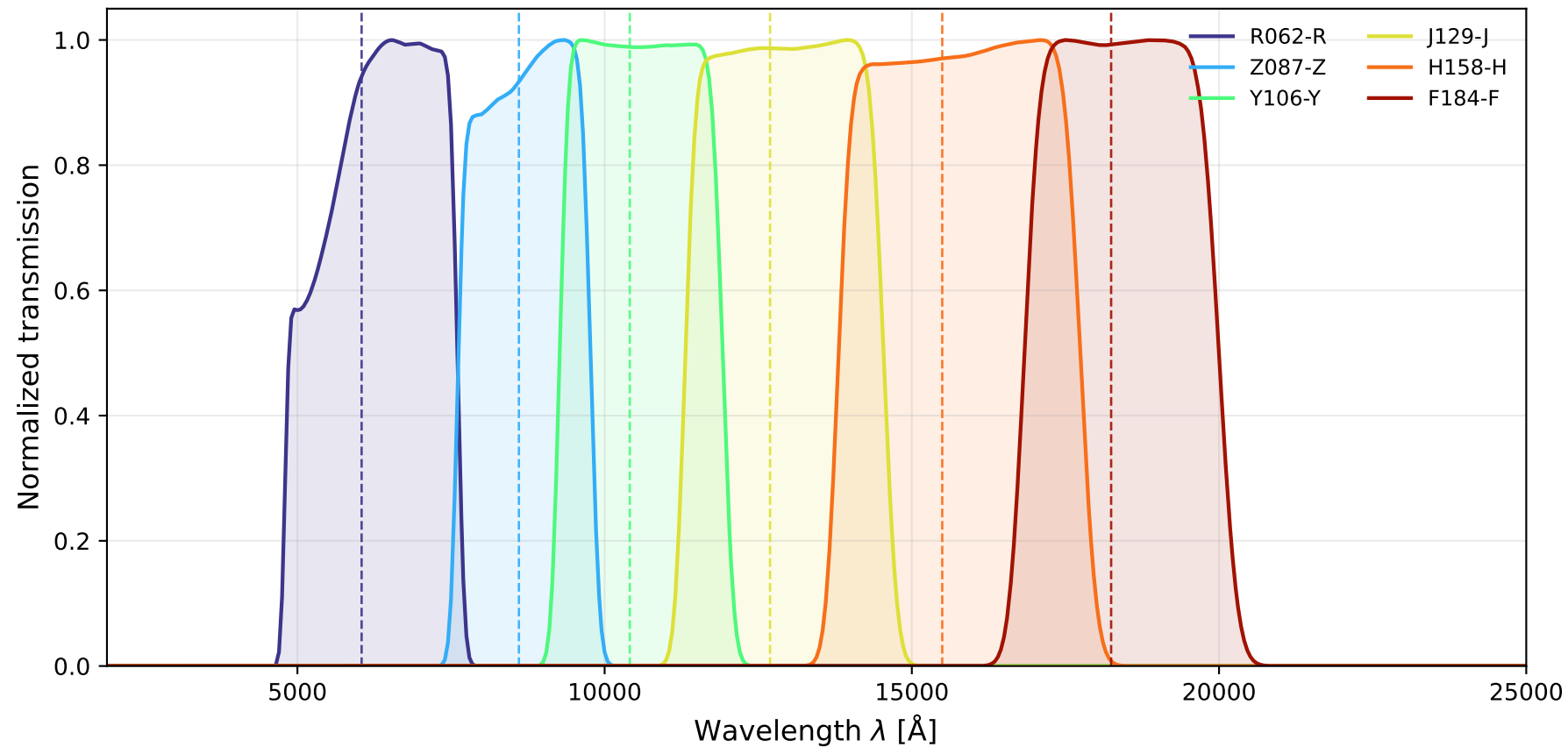
Roman filters — transmission curves and \lambda_{\text{eff}} (dashed)
