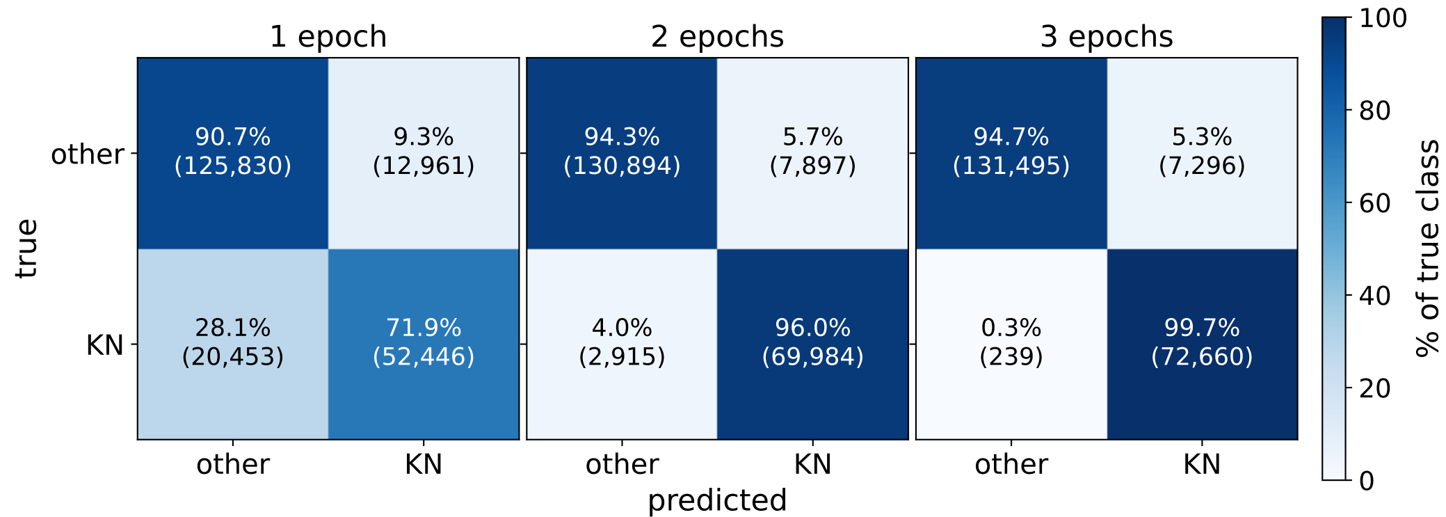
Confusion matrix (threshold=0.5, no redshift)
