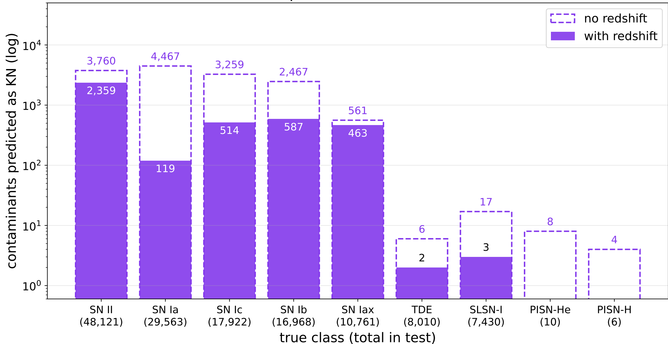
Contaminants leaking as KN by true class (2 epochs, threshold=0.2)
