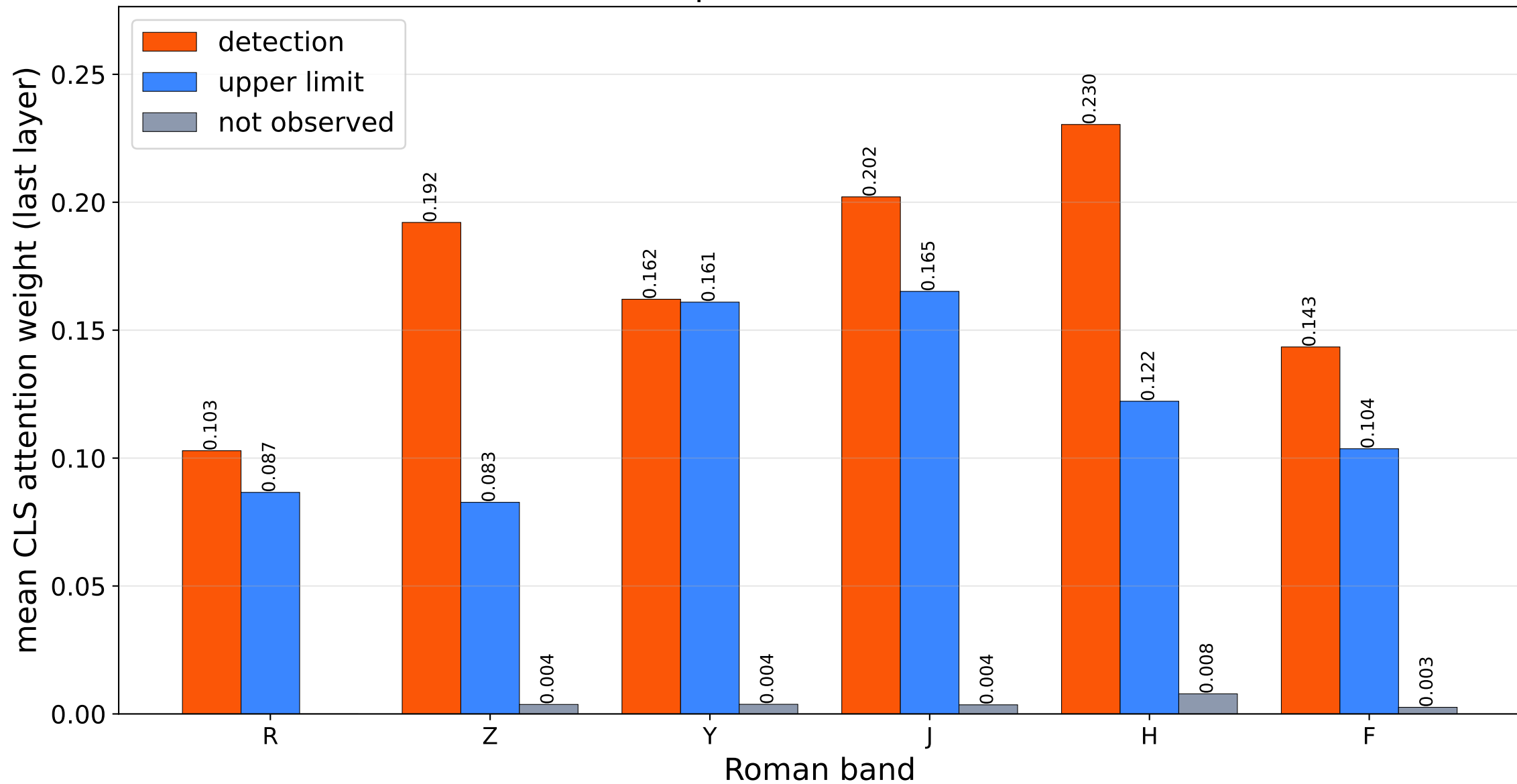
What the classifier attends to, by band and token type (2 epochs, no redshift)
