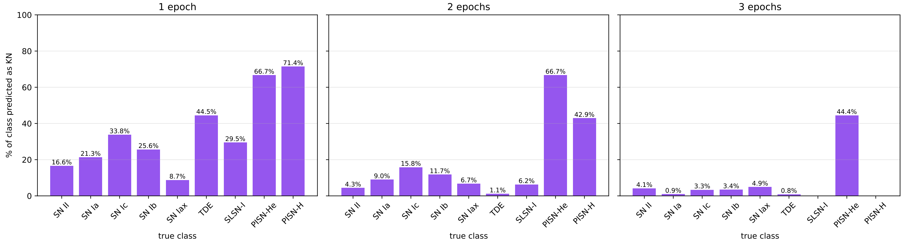
Contaminants leaking as KN by true class (threshold=0.2, no redshift)
