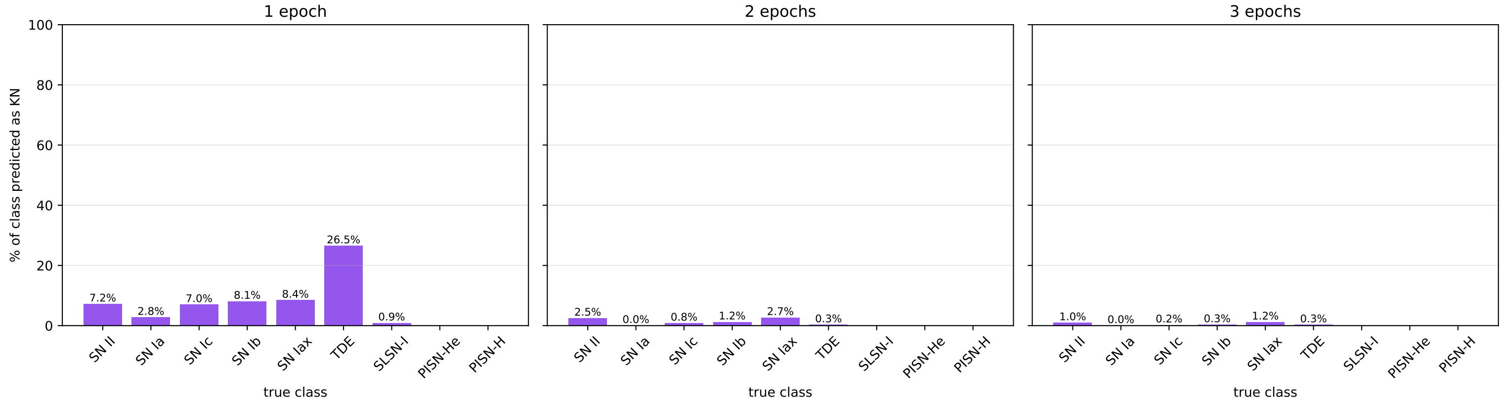
Contaminants leaking as KN by true class (threshold=0.2, with redshift)
