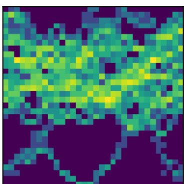
peak 27 P=2.0199d (LS)
