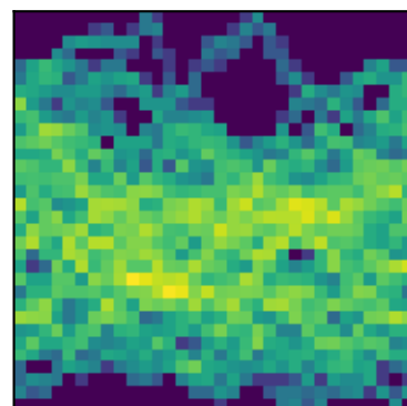
peak 29 P=2.9250d (LS)
