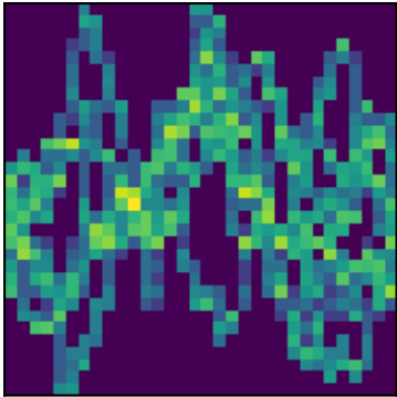
peak 16 P=2.3034d (LS)
