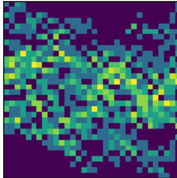
peak 17 P=0.8437d (LS)
