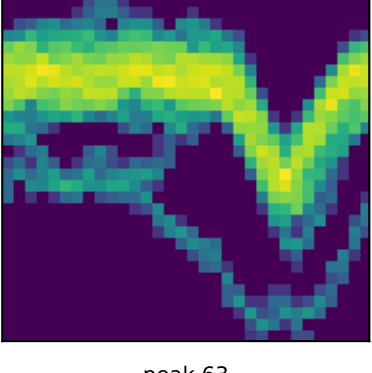
peak 63 P=1.0417d (ACF)
