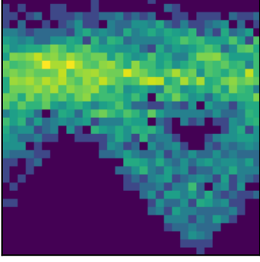
peak 20 P=0.9877d (LS)
