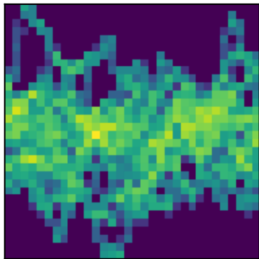
peak 43 P=1.3839d (LS)
