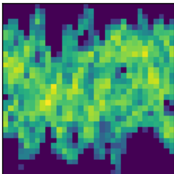
peak 19 P=1.9537d (ACF)
