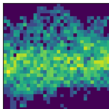
peak 22 P=1.1327d (LS)
