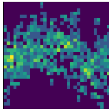
peak 10 P=7.0311d (LS)
