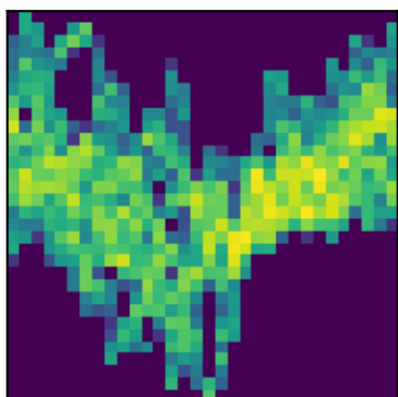
peak 26 P=1.1029d (LS)
