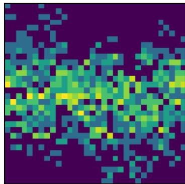
peak 9 P=4.7238d (LS)
