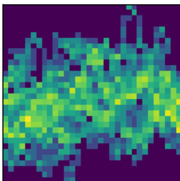
peak 29 P=4.6470d (LS)
