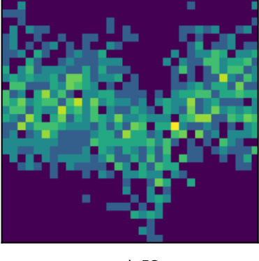
peak 52 P=3.3446d (LS)
