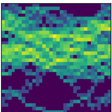
peak 20 P=1.1519d (LS)
