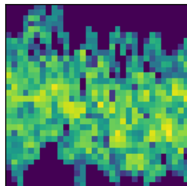
peak 28 P=1.8182d (LS)
