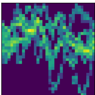
peak 30 P=3.3994d (LS)
