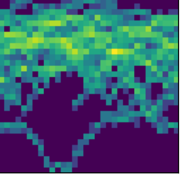
peak 41 P=6.0637d (LS)
