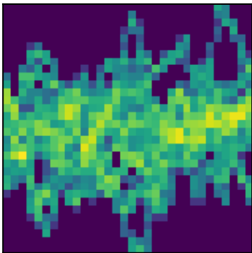
peak 44 P=1.7298d (LS)
