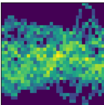
peak 24 P=1.7426d (LS)
