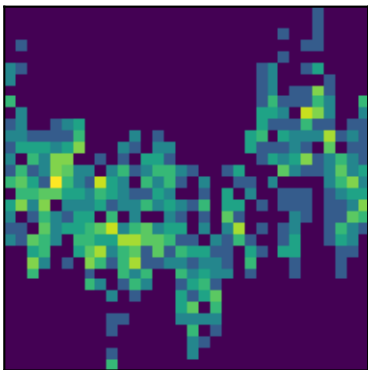
peak 14 P=0.7186d (LS)
