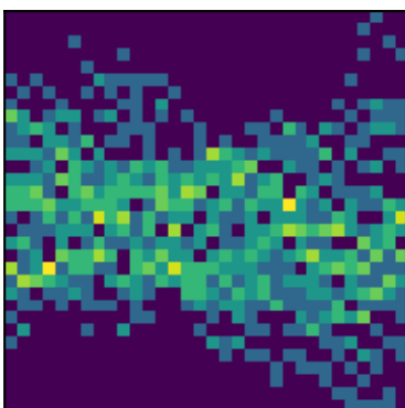
peak 6 P=3.4703d (LS)
