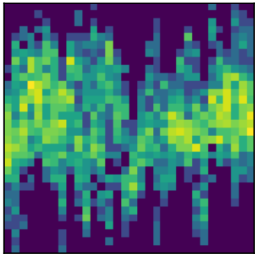
peak 33 P=7.5960d (LS)
