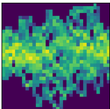
peak 24 P=0.7645d (LS)
