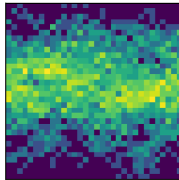
peak 17 P=0.6149d (LS)
