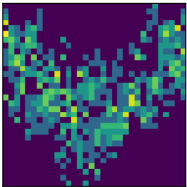
peak 13 P=0.4806d (LS)
