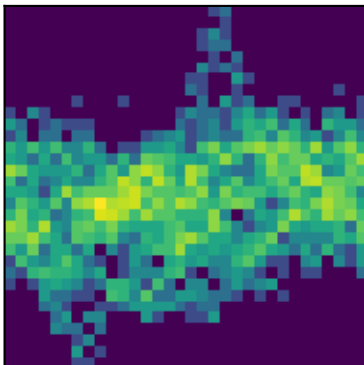
peak 32 P=5.5224d (LS)
