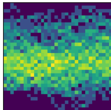
peak 16 P=0.7255d (LS)
