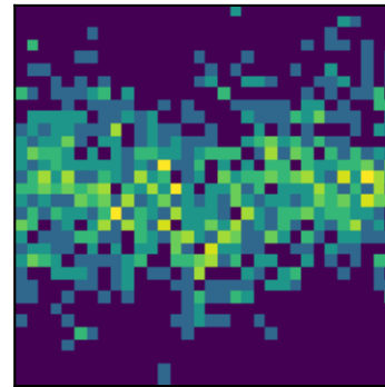
peak 4 P=1.7811d (LS)
