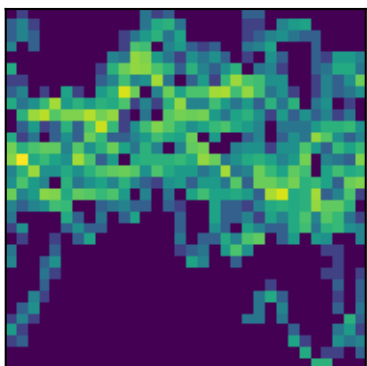
peak 33 P=6.3352d (LS)
