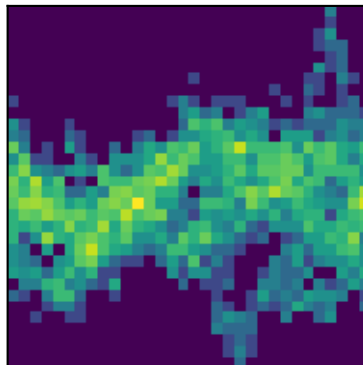
peak 35 P=0.9993d (LS)
