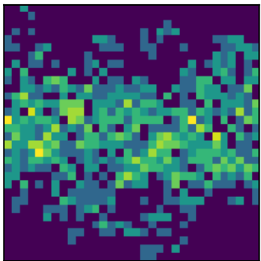
peak 7 P=2.9605d (LS)
