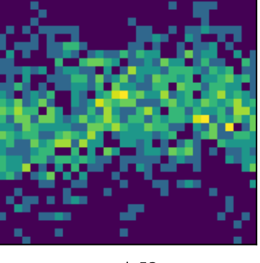
peak 53 P=7.2795d (LS)
