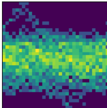
peak 22 P=1.2656d (LS)
