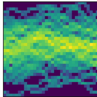
peak 17 P=1.1635d (LS)
