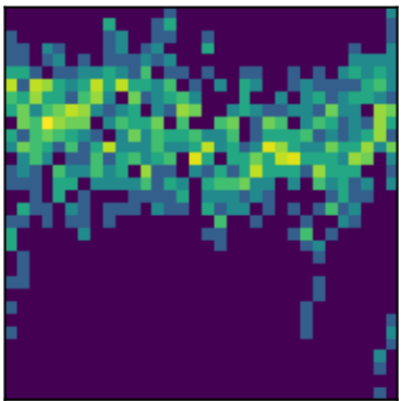
peak 14 P=0.4891d (LS)
