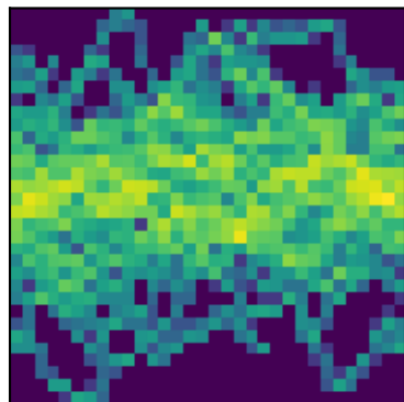
peak 21 P=5.5267d (LS)
