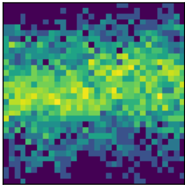
peak 18 P=0.6457d (LS)
