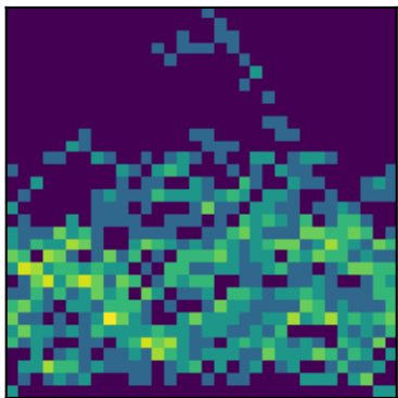
peak 9 P=4.1846d (LS)
