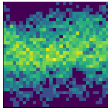
peak 16 P=0.5843d (LS)
