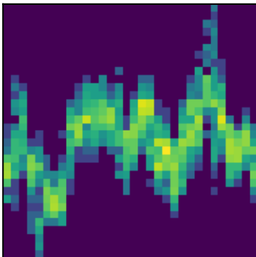
peak 39 P=2.6022d (LS)
