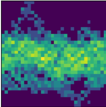
peak 26 P=1.8408d (LS)
