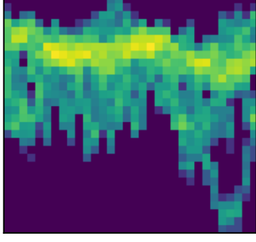
peak 61 P=2.8630d (LS)
