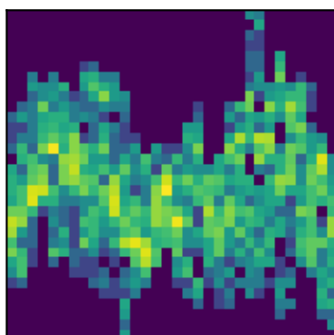
peak 34 P=0.4295d (LS)
