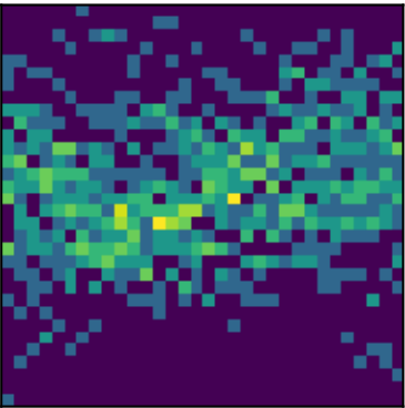
peak 6 P=2.5643d (LS)
