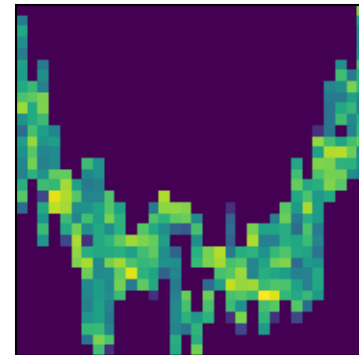
peak 17 P=8.3032d (LS)
