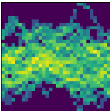
peak 20 P=1.2674d (LS)
