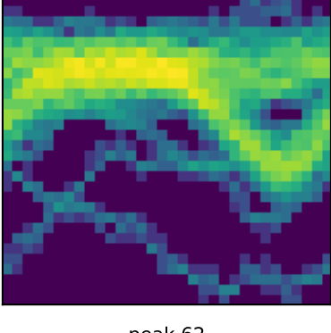
peak 62 P=6.7280d (LS)
