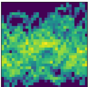
peak 25 P=0.9821d (LS)
