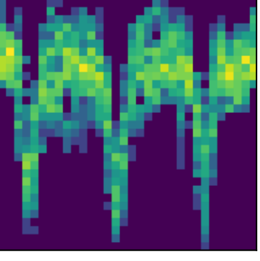
peak 35 P=1.4344d (LS)
