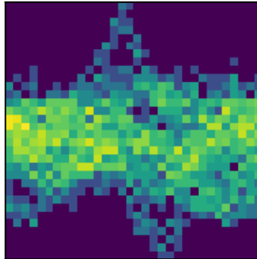
peak 29 P=2.5850d (LS)
