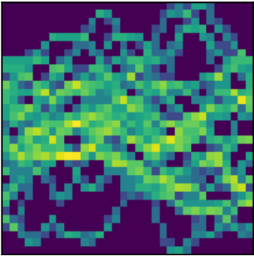
peak 8 P=2.5320d (LS)
