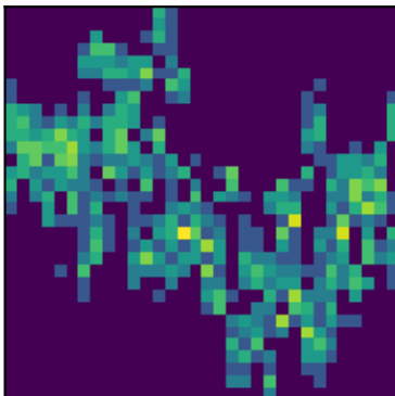
peak 20 P=1.0041d (LS)
