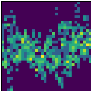
peak 13 P=0.6514d (LS)
