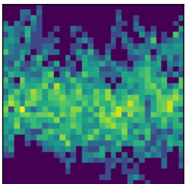
peak 31 P=7.1740d (LS)
