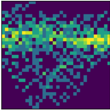
peak 7 P=1.3081d (LS)
