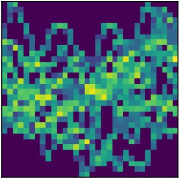
peak 13 P=1.5855d (LS)
