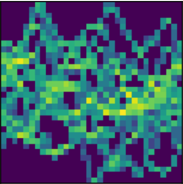
peak 12 P=7.5961d (LS)
