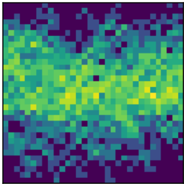
peak 21 P=0.7732d (LS)
