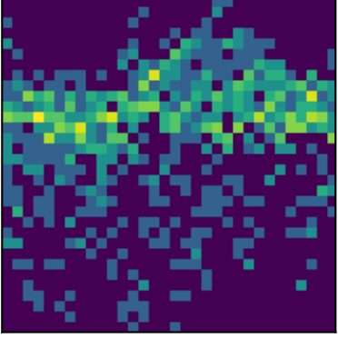
peak 15 P=0.5077d (LS)
