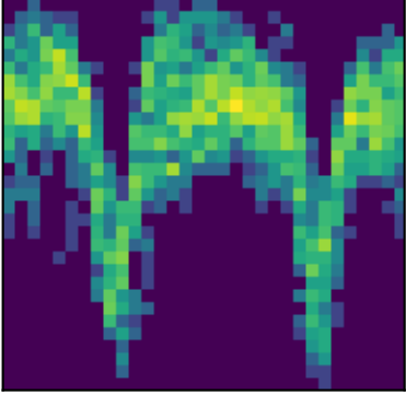
peak 34 P=1.0422d (LS)
