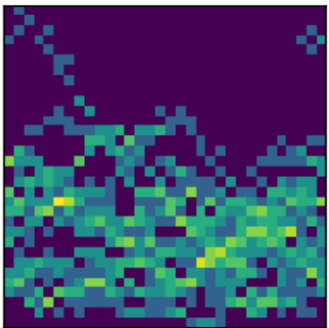
peak 8 P=3.4673d (LS)
