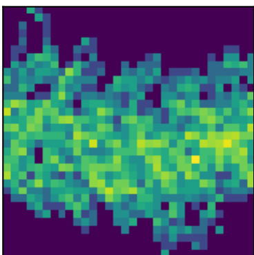
peak 26 P=2.3235d (LS)
