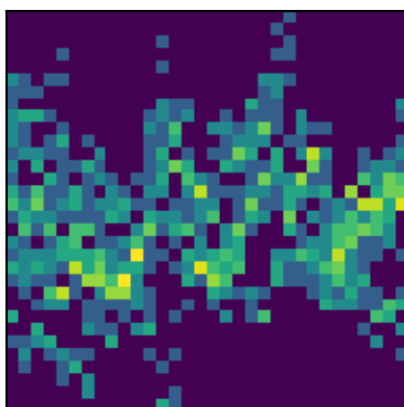
peak 11 P=0.4647d (LS)
