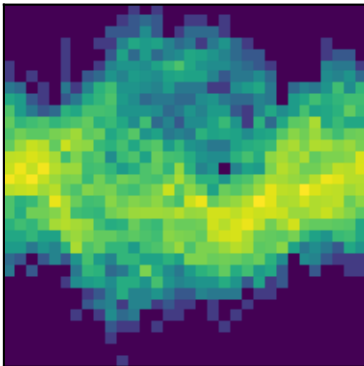
peak 37 P=1.6222d (LS)
