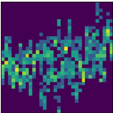
peak 15 P=0.7495d (LS)
