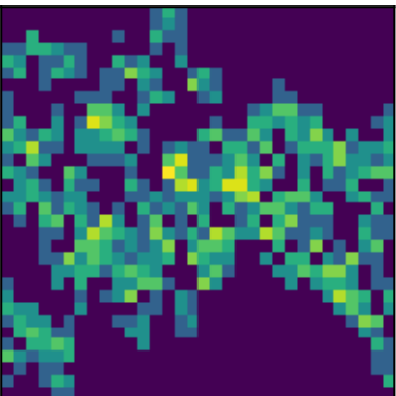
peak 18 P=0.8933d (LS)
