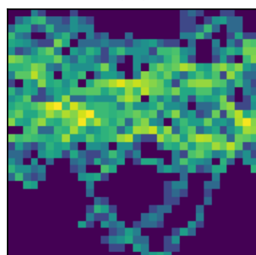
peak 28 P=2.4030d (LS)
