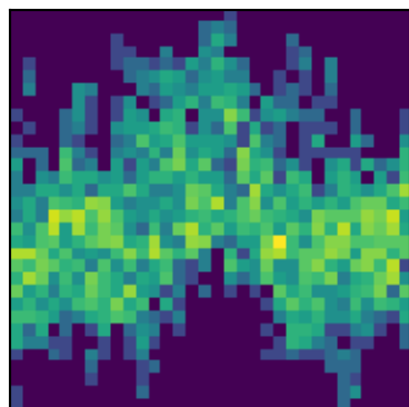
peak 27 P=2.4833d (LS)
