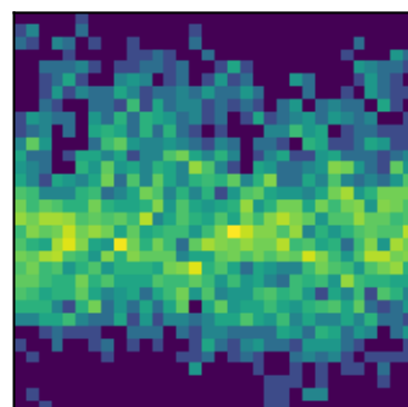
peak 23 P=1.2537d (LS)
