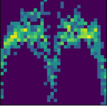
peak 18 P=0.9030d (LS)
