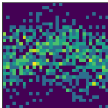
peak 6 P=1.8750d (LS)
