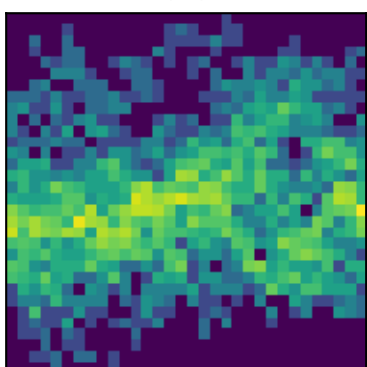
peak 24 P=1.3313d (LS)
