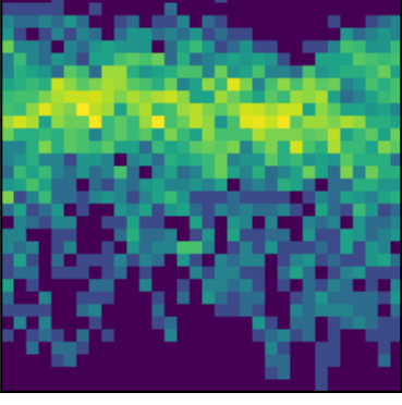
peak 24 P=1.2395d (LS)
