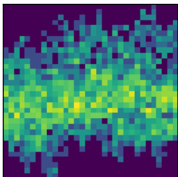
peak 26 P=1.5192d (LS)
