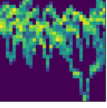
peak 47 P=1.1049d (LS)
