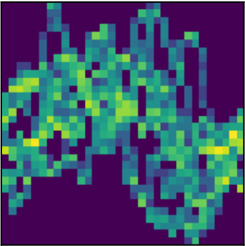
peak 15 P=2.0347d (LS)
