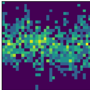
peak 8 P=4.1787d (LS)
