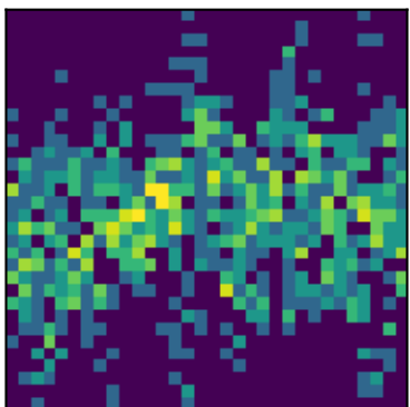
peak 13 P=0.4818d (LS)
