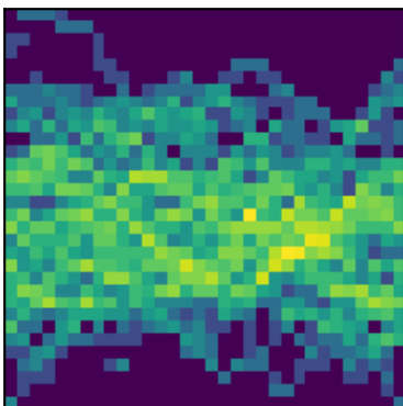
peak 18 P=0.9549d (LS)
