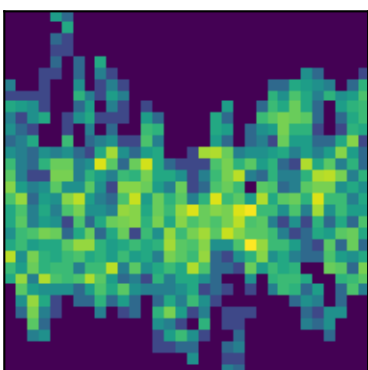
peak 32 P=0.3375d (LS)
