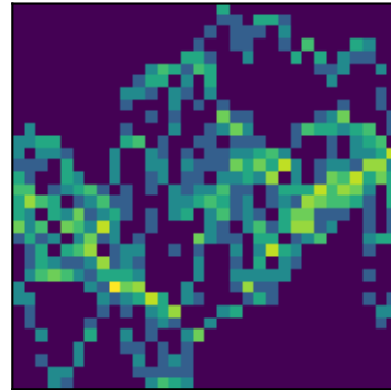
peak 9 P=8.6756d (LS)
