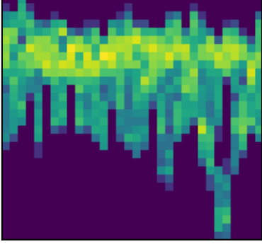
peak 62 P=6.7280d (LS)
