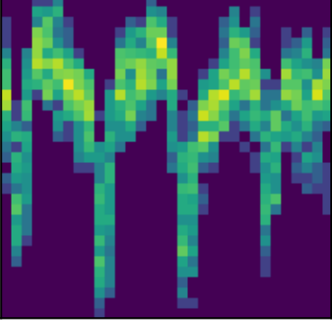
peak 36 P=1.9618d (LS)
