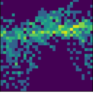
peak 12 P=2.0833d (ACF)
