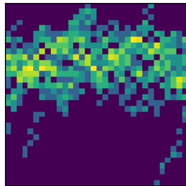
peak 10 P=0.4035d (LS)
