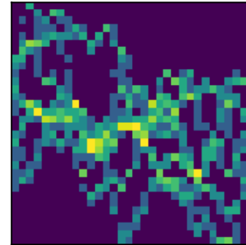
peak 10 P=0.6453d (LS)
