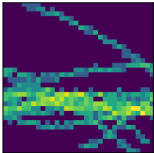
peak 0 P=1.8397\text{d} (LS)
