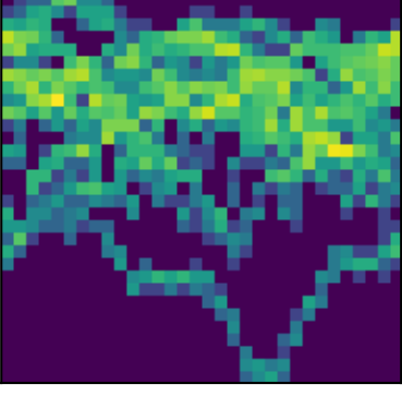
peak 42 P=11.1167d (LS)
