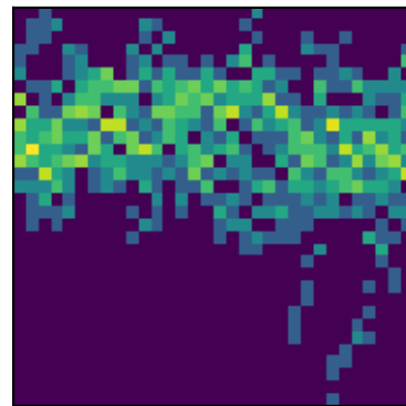
peak 11 P=0.4179d (LS)
