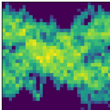
peak 15 P=1.0390d (LS)
