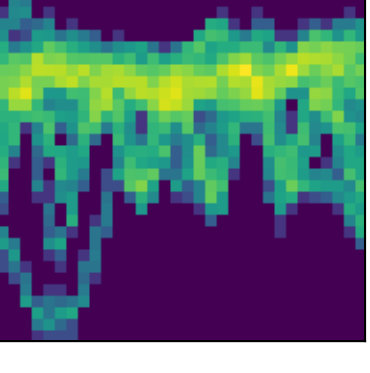
peak 59 P=1.7475d (LS)
