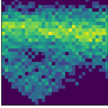
peak 19 P=0.9506d (LS)
