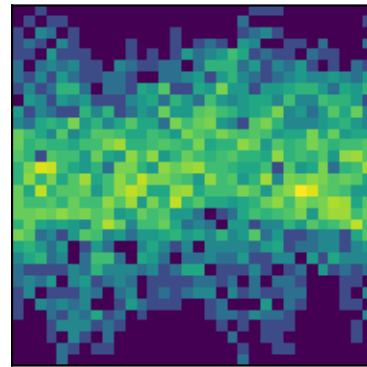
peak 23 P=0.9158d (LS)
