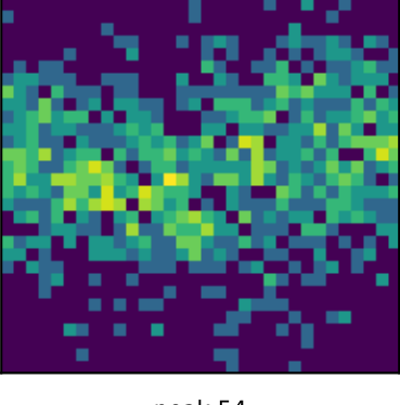
peak 54 P=0.2613d (LS)
