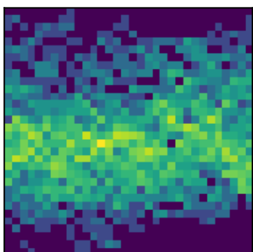
peak 18 P=0.7826d (LS)
