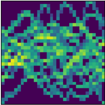
peak 10 P=3.6895d (LS)
