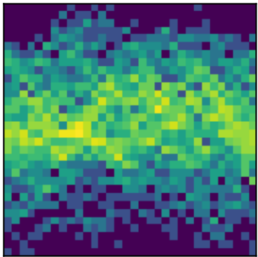
peak 19 P=0.6980d (LS)
