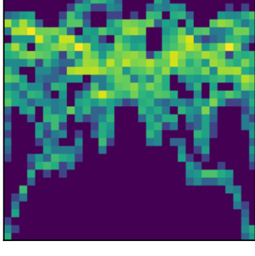
peak 43 P=1.0347d (ACF)
