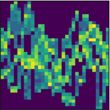
peak 17 P=2.9776d (LS)
