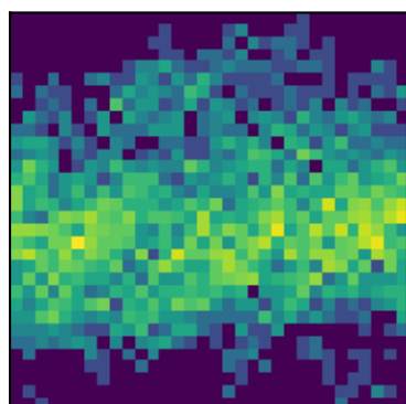
peak 21 P=1.0499d (LS)
