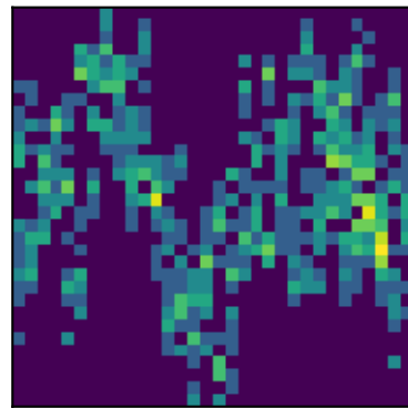
peak 16 P=0.9341d (LS)
