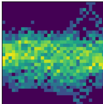
peak 23 P=1.3806d (LS)
