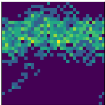
peak 6 P=2.4692d (LS)
