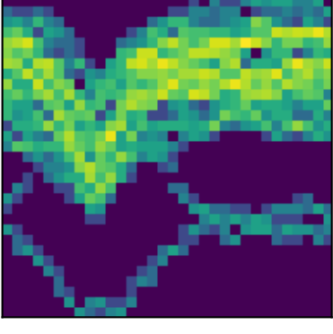
peak 40 P=4.7643d (LS)
