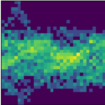
peak 27 P=2.0592d (LS)
