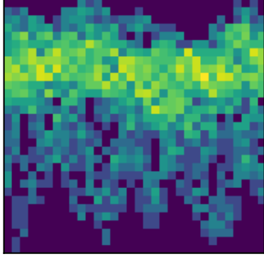
peak 31 P=0.3483d (LS)
