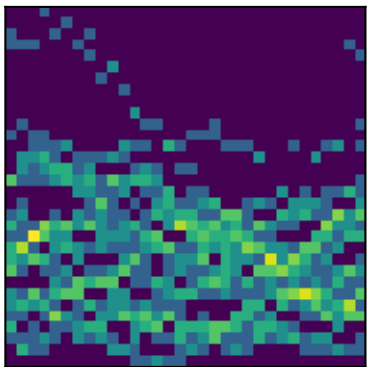
peak 7 P=3.0339d (LS)
