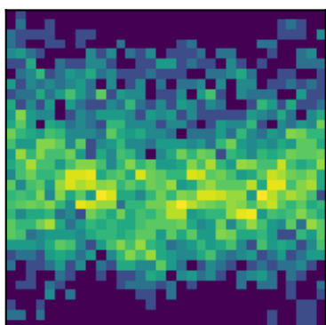
peak 20 P=0.9565d (LS)
