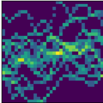
peak 7 P=4.8584d (LS)
