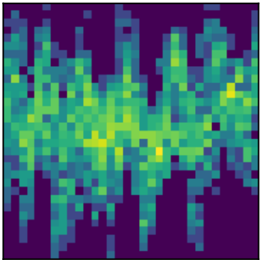
peak 32 P=4.9666d (LS)
