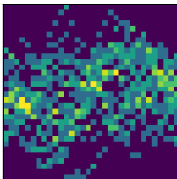
peak 9 P=3.6291d (LS)
