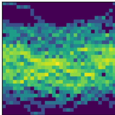
peak 16 P=0.8201d (LS)
