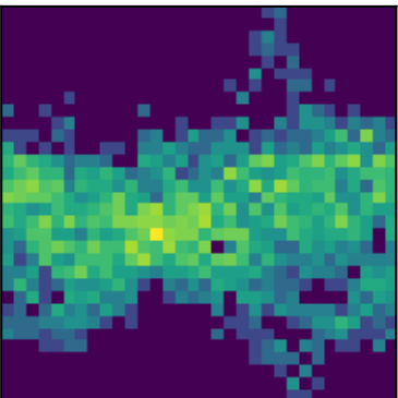
peak 30 P=3.2836d (LS)
