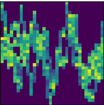
peak 18 P=3.8151d (LS)
