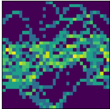
peak 6 P=3.7956d (LS)
