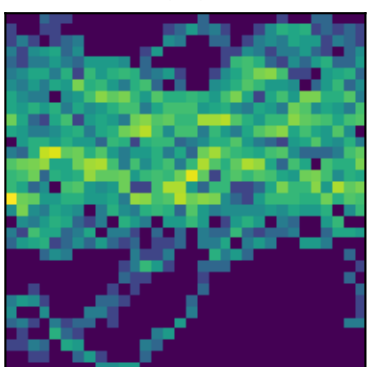
peak 25 P=1.6792d (LS)
