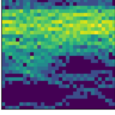
peak 37 P=2.6157d (LS)
