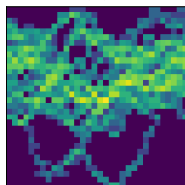
peak 29 P=2.6803d (LS)
