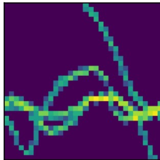
peak 4 P=6.0300\text{d} (LS)
