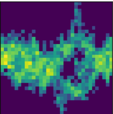
peak 36 P=1.1152d (LS)
