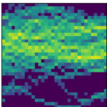
peak 18 P=1.0324d (LS)
