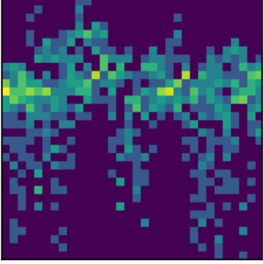
peak 16 P=0.5224d (LS)
