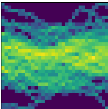
peak 38 P=0.5661d (LS)
