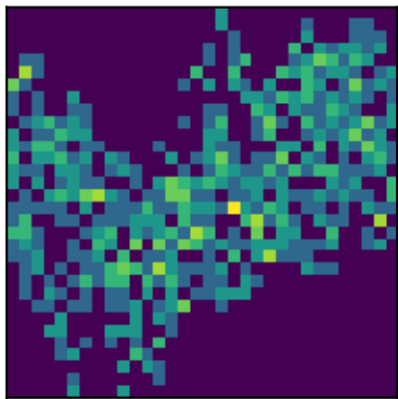
peak 12 P=0.3867d (LS)
