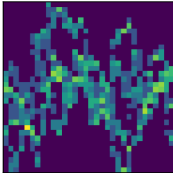
peak 13 P=1.2581d (LS)
