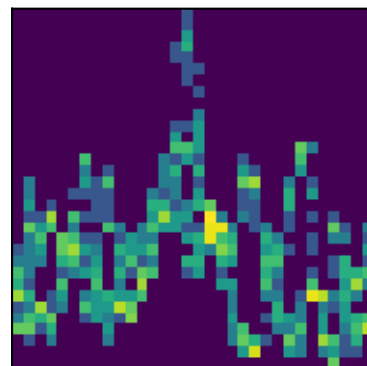
peak 17 P=0.9481d (LS)
