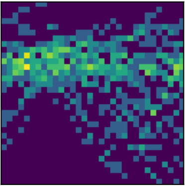
peak 9 P=1.5411d (LS)
