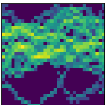
peak 24 P=1.5660d (LS)
