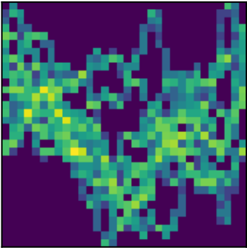
peak 14 P=1.8221d (LS)
