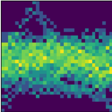
peak 25 P=1.6643d (LS)
