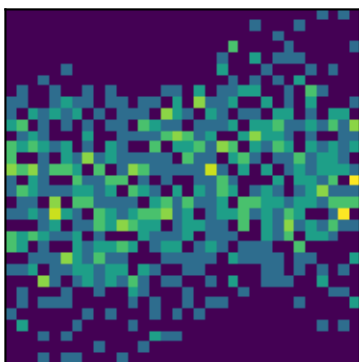
peak 7 P=2.1227d (LS)
