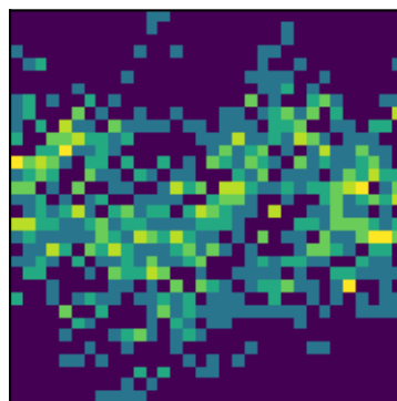
peak 10 P=0.3412d (LS)
