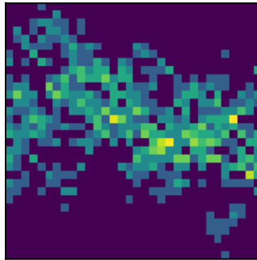
peak 10 P=8.6087d (LS)
