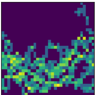
peak 13 P=0.5444d (LS)
