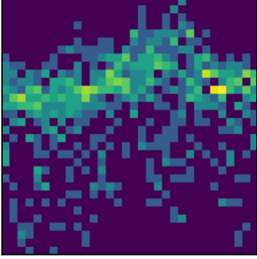
peak 14 P=0.3483d (LS)
