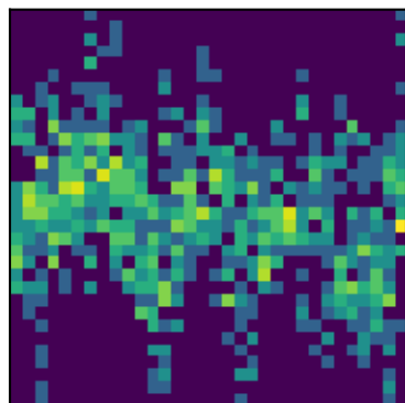
peak 15 P=0.6869d (LS)
