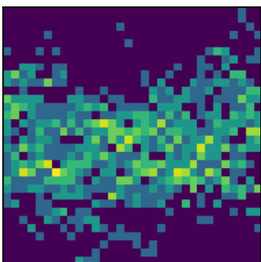
peak 8 P=6.3926d (LS)
