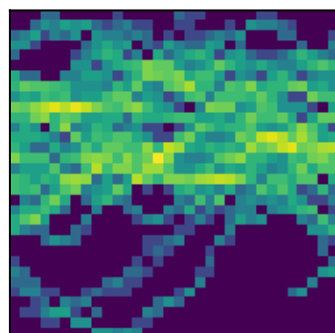
peak 22 P=1.2787d (LS)
