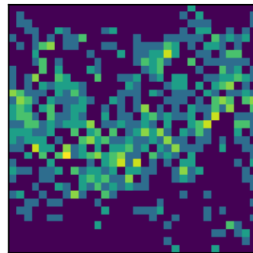
peak 11 P=0.3634d (LS)
