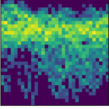
peak 28 P=2.0972d (ACF)
