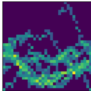
peak 10 P=5.0564d (LS)
