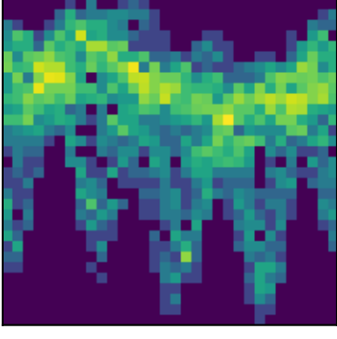
peak 32 P=0.5231d (LS)
