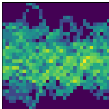
peak 22 P=1.4522d (LS)
