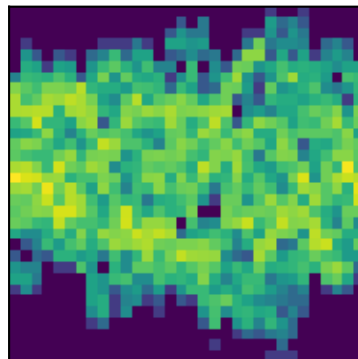
peak 16 P=1.4503d (LS)
