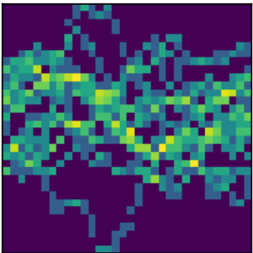
peak 19 P=6.4254d (LS)
