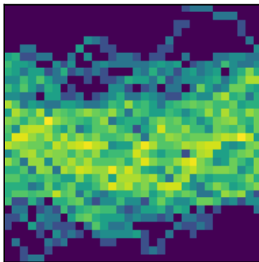
peak 17 P=0.8823d (LS)
