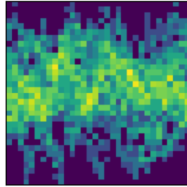
peak 29 P=1.2785d (LS)
