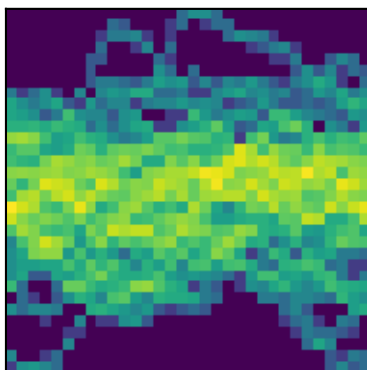
peak 41 P=0.9295d (LS)
