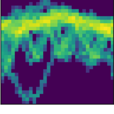
peak 58 P=1.4017d (LS)
