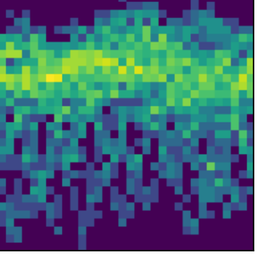
peak 29 P=3.1320d (ACF)
