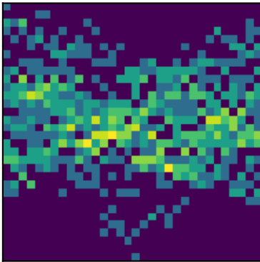
peak 7 P=3.0130d (LS)
