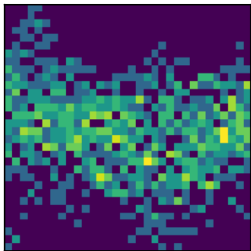
peak 8 P=3.6216d (LS)
