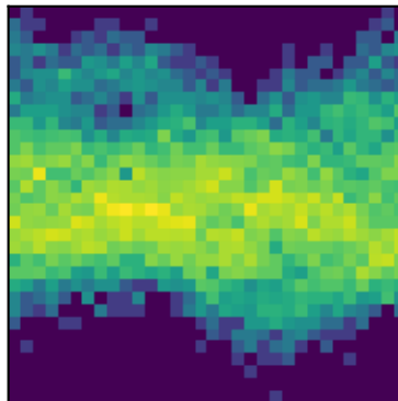
peak 41 P=8.9219d (LS)
