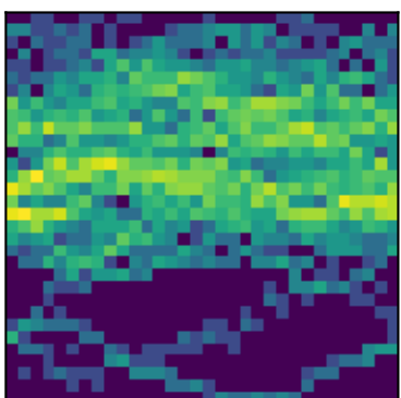
peak 19 P=1.0889d (LS)
