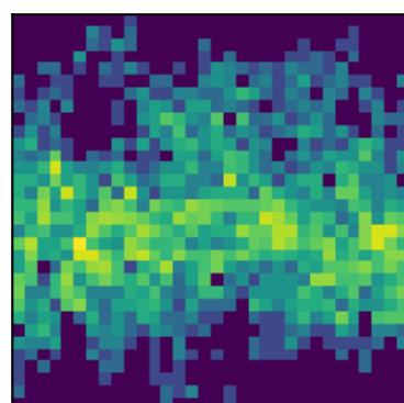
peak 28 P=2.8696d (LS)
