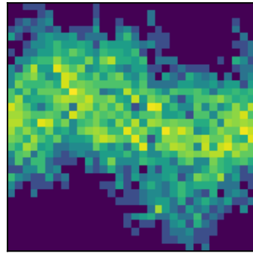
peak 28 P=1.2182d (LS)
