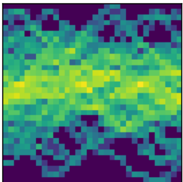
peak 19 P=2.1054d (LS)
