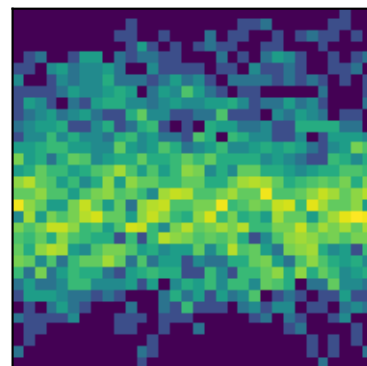
peak 17 P=0.7508d (LS)
