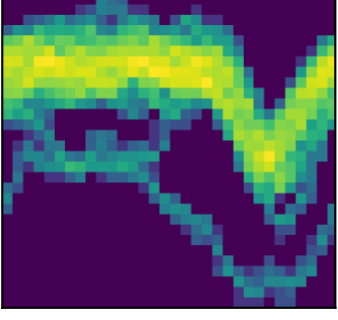
peak 63 P=1.0417d (ACF)
