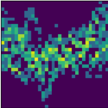
peak 13 P=5.2762d (LS)
