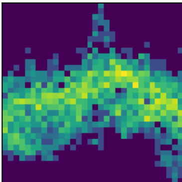
peak 33 P=8.0996d (LS)
