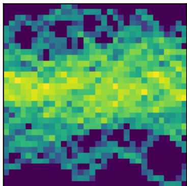
peak 20 P=2.9476d (LS)
