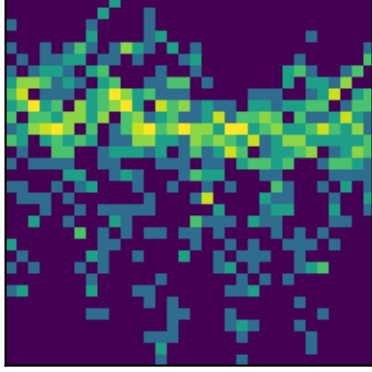
peak 13 P=0.2612d (LS)
