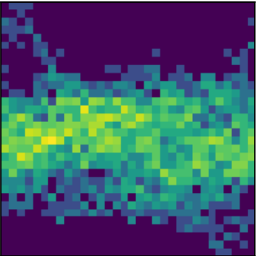
peak 24 P=1.5187d (LS)
