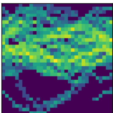
peak 21 P=1.2120d (LS)
