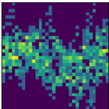
peak 12 P=0.4679d (LS)
