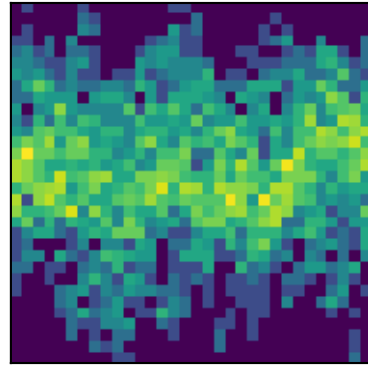
peak 34 P=0.8194d (ACF)
