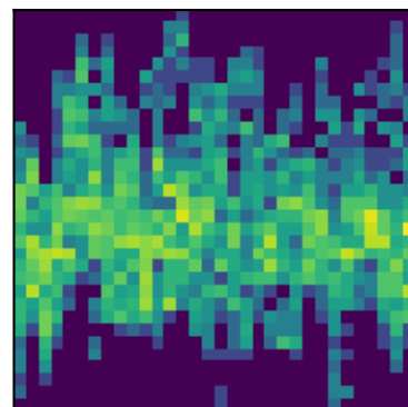
peak 29 P=3.3982d (LS)
