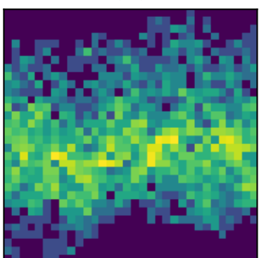
peak 25 P=1.4190d (LS)
