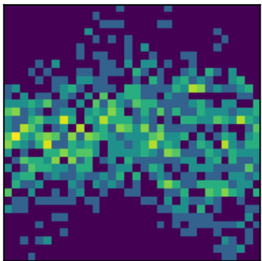
peak 7 P=2.9364d (LS)
