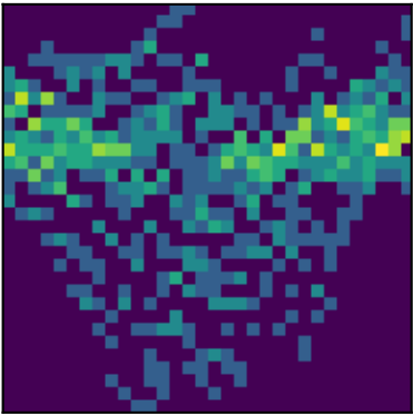
peak 10 P=3.4091d (LS)
