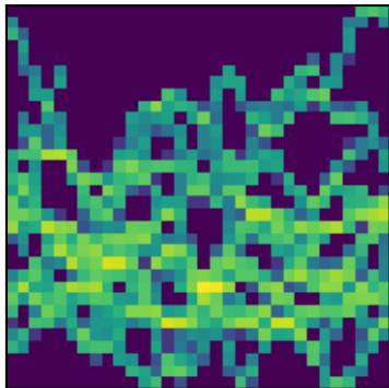
peak 14 P=1.7298d (LS)
