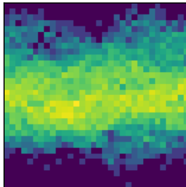
peak 40 P=3.9034d (LS)
