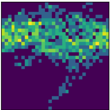
peak 8 P=3.5047d (LS)
