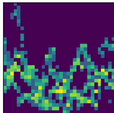
peak 16 P=0.8551d (LS)
