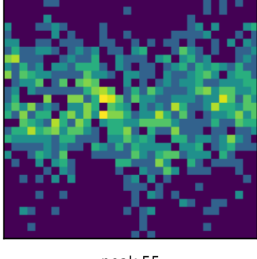
peak 55 P=0.3486d (LS)
