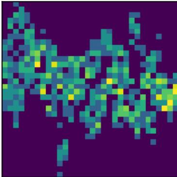
peak 15 P=0.6328d (LS)
