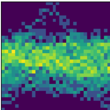
peak 21 P=1.1355d (LS)
