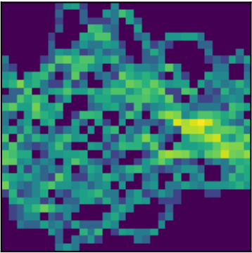
peak 9 P=3.0031d (LS)
