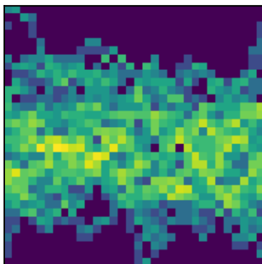
peak 23 P=1.5664d (LS)
