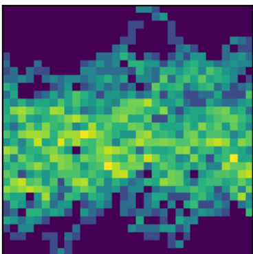
peak 21 P=1.3668d (LS)
