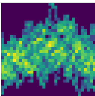
peak 30 P=7.3373d (LS)
