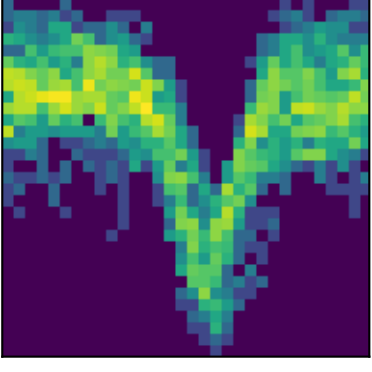
peak 33 P=0.9882d (LS)
