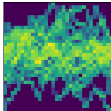
peak 23 P=0.5953d (LS)
