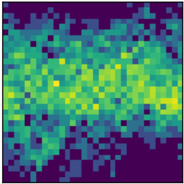
peak 25 P=1.0010d (LS)
