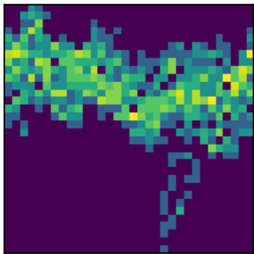
peak 12 P=0.4276d (LS)
