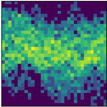
peak 27 P=1.1530d (LS)
