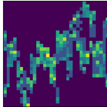
peak 15 P=2.1850d (LS)
