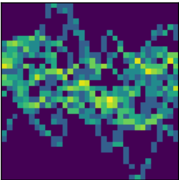
peak 20 P=8.1388d (LS)
