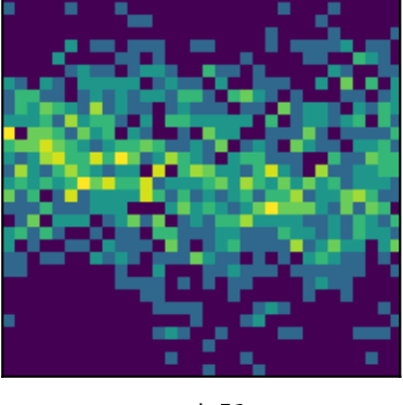
peak 51 P=2.8125d (LS)
