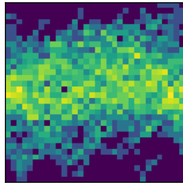
peak 22 P=0.8173d (LS)
