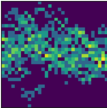
peak 8 P=3.7663d (LS)
