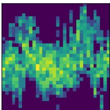
peak 30 P=4.9666d (LS)
