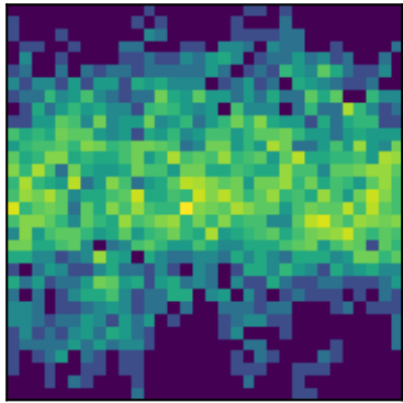
peak 24 P=0.9565d (LS)
