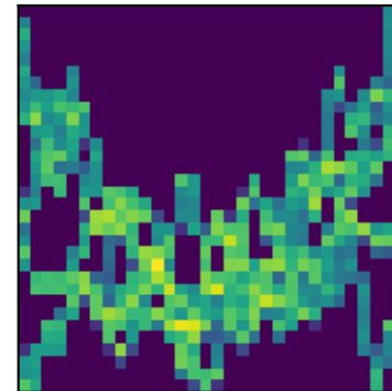
peak 16 P=4.1516d (LS)
