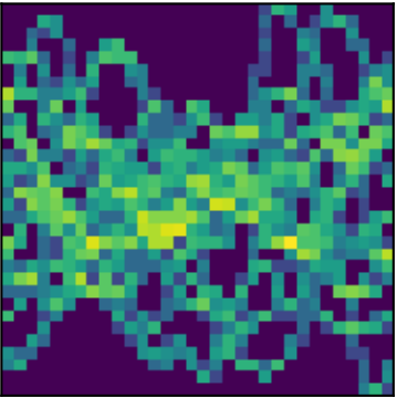
peak 11 P=5.3806d (LS)
