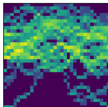
peak 23 P=1.4671d (LS)
