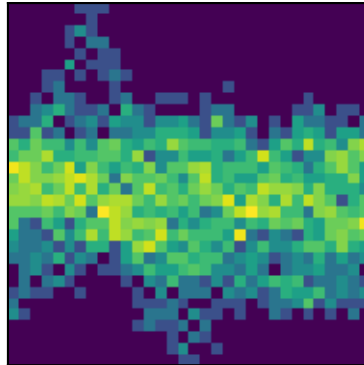
peak 28 P=2.2923d (LS)
