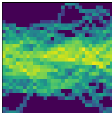
peak 40 P=0.8415d (LS)
