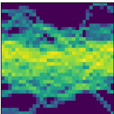
peak 39 P=0.7241d (LS)
