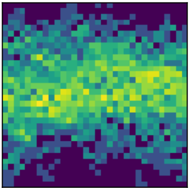
peak 20 P=0.7337d (LS)
