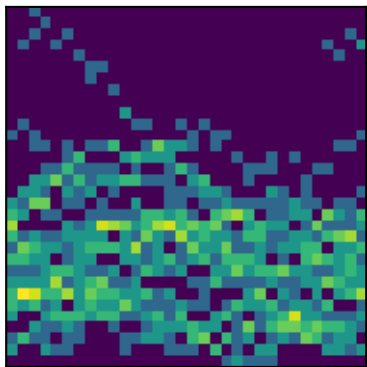
peak 6 P=2.4766d (LS)
