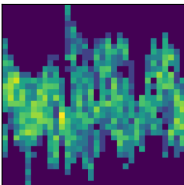
peak 36 P=0.4827d (LS)
