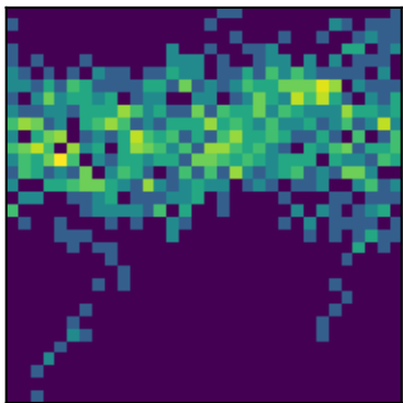
peak 9 P=6.3910d (LS)
