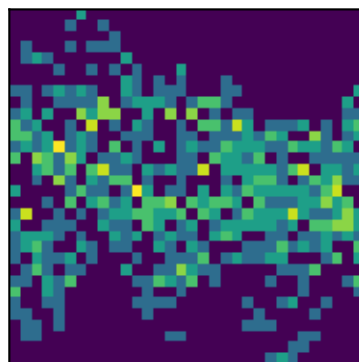
peak 11 P=0.3878d (LS)
