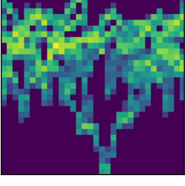
peak 46 P=1.0487d (LS)
