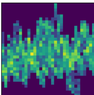
peak 35 P=0.4546d (LS)
