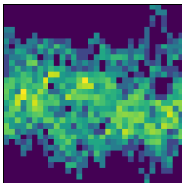
peak 28 P=3.5746d (LS)
