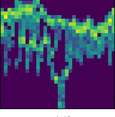
peak 48 P=1.4390d (LS)
