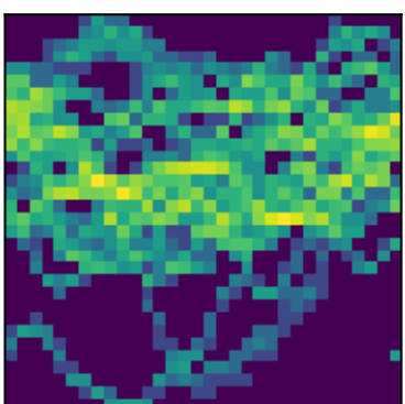
peak 26 P=1.7869d (LS)
