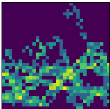
peak 12 P=0.5299d (LS)
