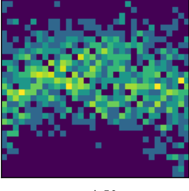
peak 50 P=2.4265d (LS)
