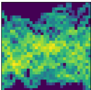
peak 30 P=7.9146d (LS)
