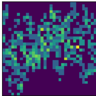
peak 15 P=0.7802d (LS)
