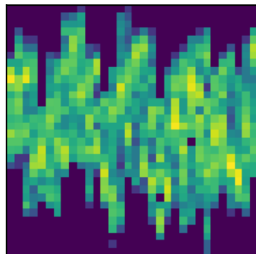
peak 18 P=8.7015d (LS)
