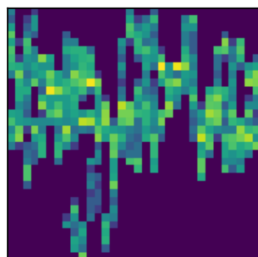
peak 34 P=8.7109d (LS)
