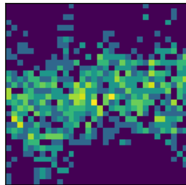
peak 10 P=0.2922d (LS)
