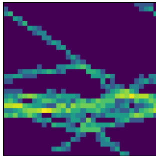
peak 1 P=2.2151\text{d} (LS)
