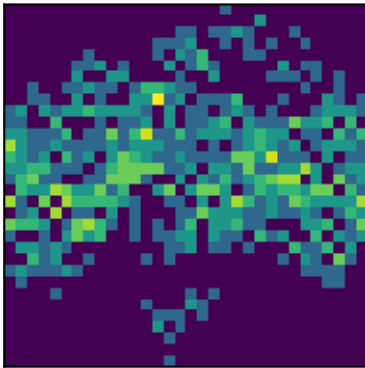
peak 9 P=5.7391d (LS)
