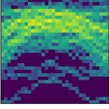
peak 38 P=3.1762d (LS)
