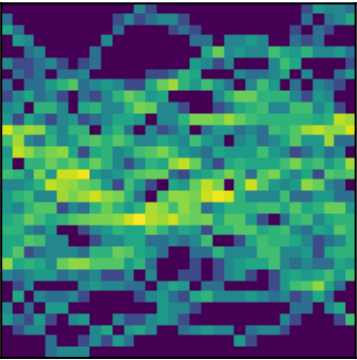
peak 6 P=1.8188d (LS)
