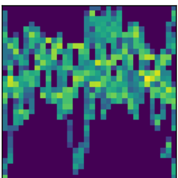
peak 32 P=4.9777d (LS)
