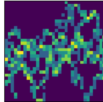
peak 11 P=0.9025d (LS)
