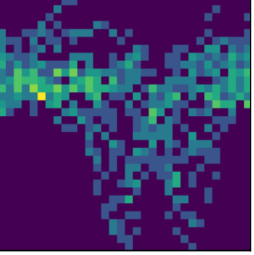
peak 17 P=0.5403d (LS)
