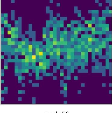
peak 56 P=0.5236d (LS)
