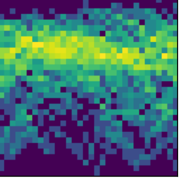
peak 23 P=1.1706d (LS)
