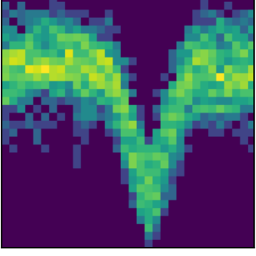
peak 27 P=1.0486d (ACF)
