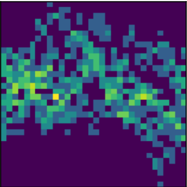
peak 12 P=4.0451d (LS)
