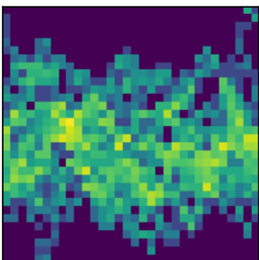
peak 27 P=2.9044d (LS)
