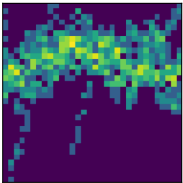
peak 13 P=0.4595d (LS)
