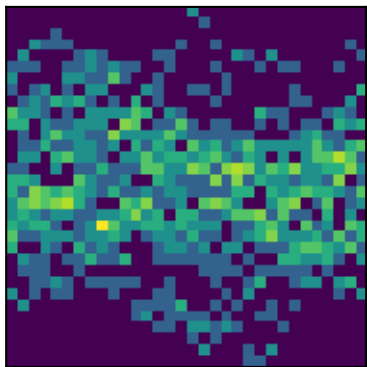
peak 6 P=2.4999d (LS)
