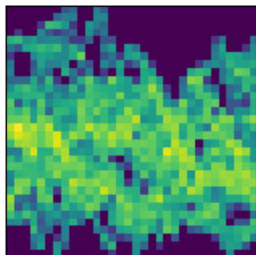
peak 27 P=1.3063d (LS)
