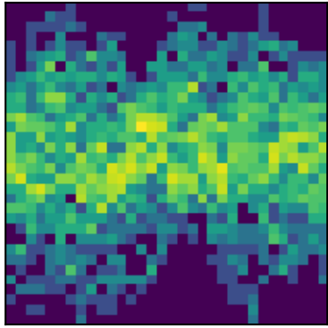
peak 30 P=1.8715d (LS)
