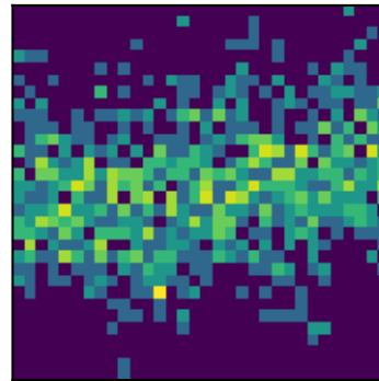
peak 5 P=1.9754d (LS)
