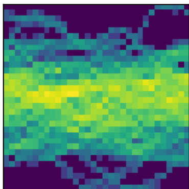
peak 37 P=0.5345d (LS)
