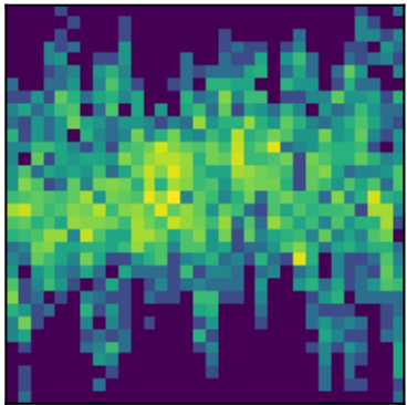
peak 31 P=2.8072d (LS)
