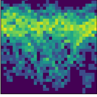
peak 26 P=1.3893d (LS)
