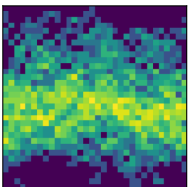
peak 19 P=0.8496d (LS)
