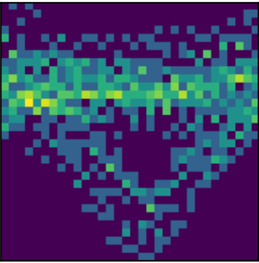
peak 6 P=1.1138d (LS)
