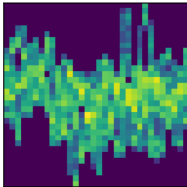
peak 46 P=4.7903d (LS)
