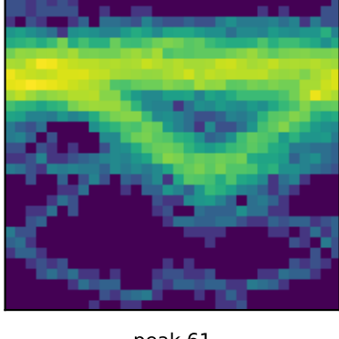
peak 61 P=2.8630d (LS)
