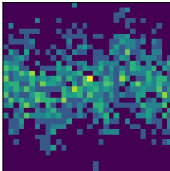
peak 7 P=2.8591d (LS)
