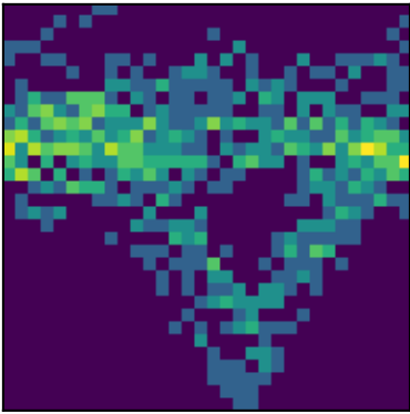
peak 8 P=1.4062d (LS)
