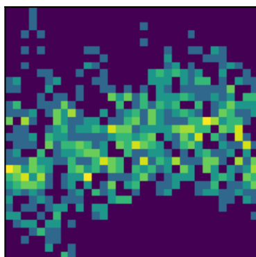
peak 10 P=0.3327d (LS)
