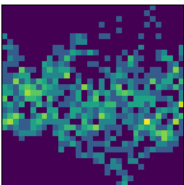
peak 9 P=10.1216d (LS)
