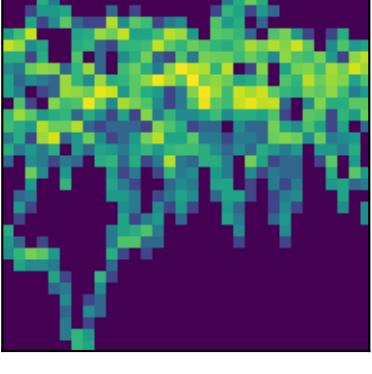
peak 45 P=0.8036d (LS)
