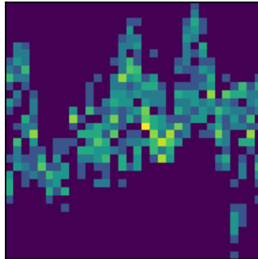
peak 16 P=0.6942d (LS)
