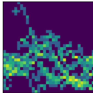
peak 11 P=9.3350d (LS)
