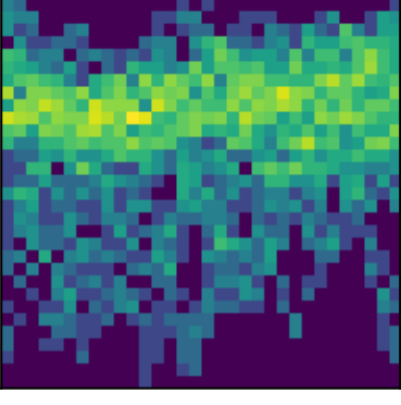
peak 30 P=4.1875d (ACF)
