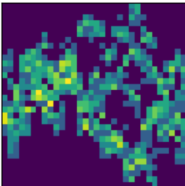
peak 19 P=0.9492d (LS)
