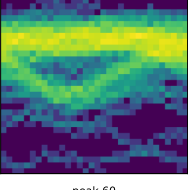
peak 60 P=2.1359d (LS)
