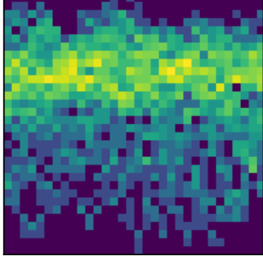
peak 25 P=1.2900d (LS)
