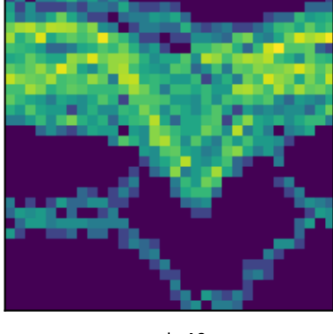
peak 49 P=1.5866d (LS)
