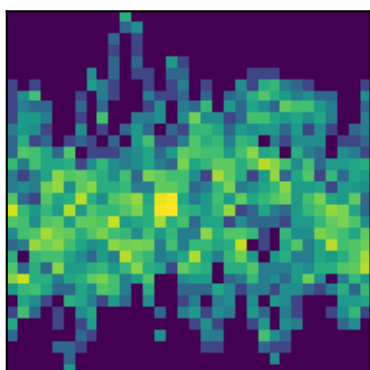
peak 31 P=0.2818d (LS)
