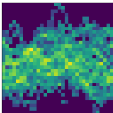
peak 25 P=2.0204d (LS)
