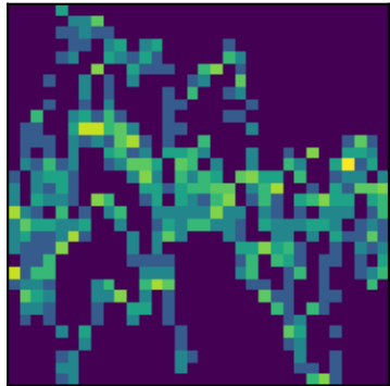
peak 12 P=1.0830d (LS)
