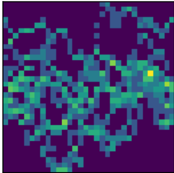
peak 8 P=6.0729d (LS)
