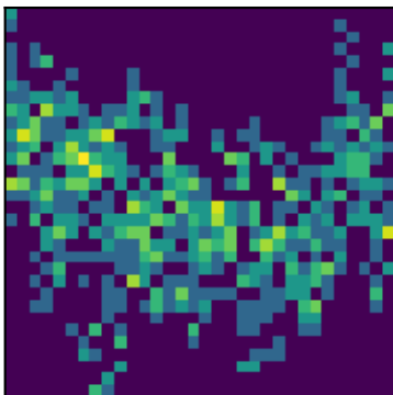
peak 14 P=0.8647d (LS)
