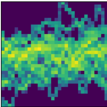
peak 42 P=1.1120d (LS)
