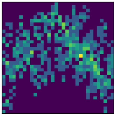
peak 14 P=0.5693d (LS)
