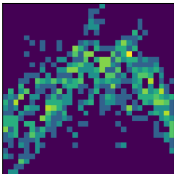
peak 13 P=0.5706d (LS)
