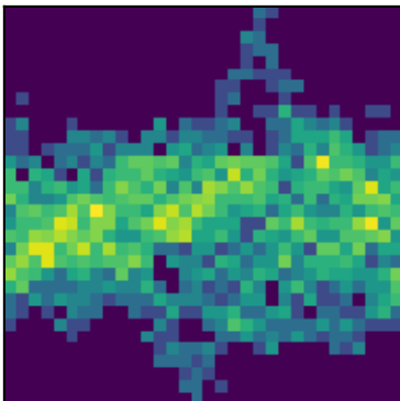
peak 31 P=4.0498d (LS)
