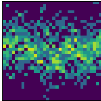
peak 6 P=2.4692d (LS)
