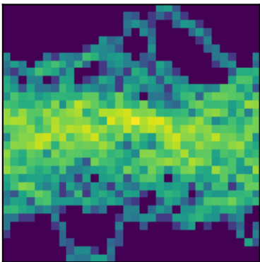
peak 45 P=2.4421d (LS)
