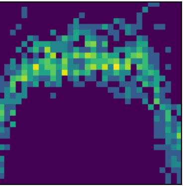
peak 11 P=1.0625d (ACF)
