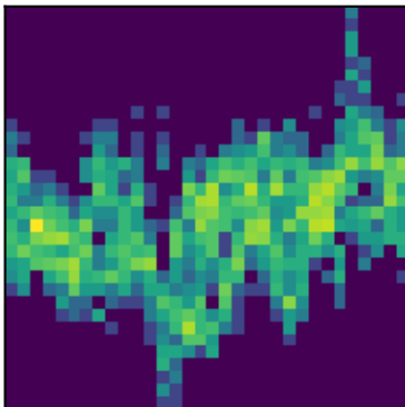
peak 38 P=1.9827d (LS)
