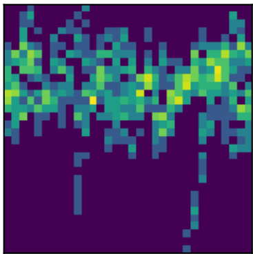
peak 15 P=0.5381d (LS)
