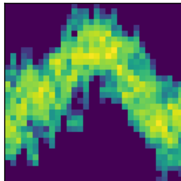
peak 17 P=2.0780d (LS)
