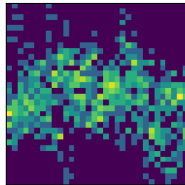
peak 11 P=0.4348d (LS)
