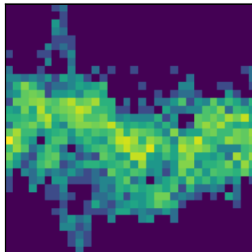
peak 34 P=0.8111d (LS)
