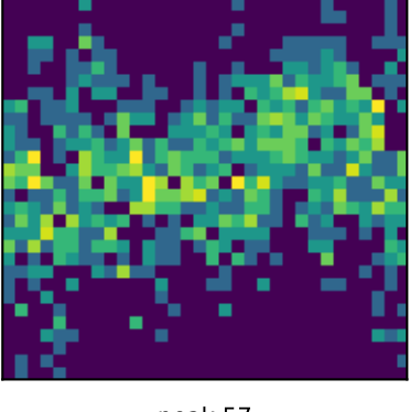
peak 57 P=1.0431d (LS)
