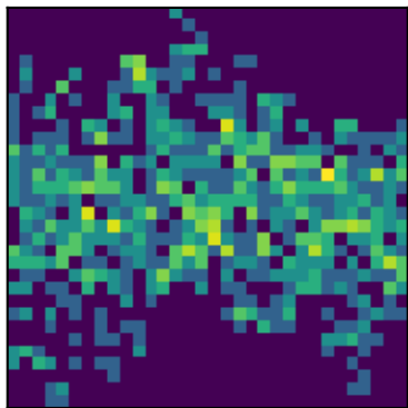
peak 8 P=3.5156d (LS)
