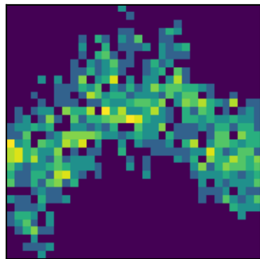
peak 9 P=4.4999d (LS)
