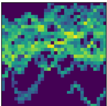
peak 31 P=4.0993d (LS)
