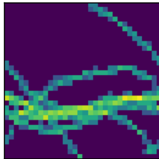
peak 2 P=2.9335\text{d} (LS)
