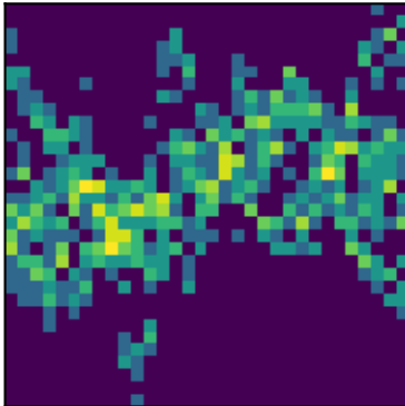
peak 14 P=8.6680d (LS)
