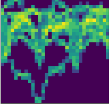
peak 44 P=0.5222d (LS)
