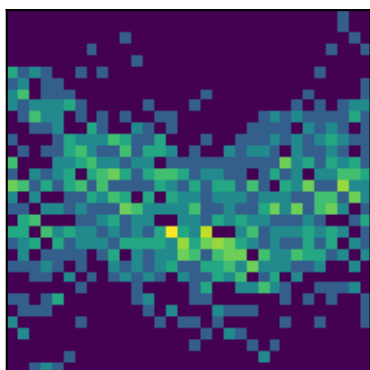
peak 7 P=4.6715d (LS)
