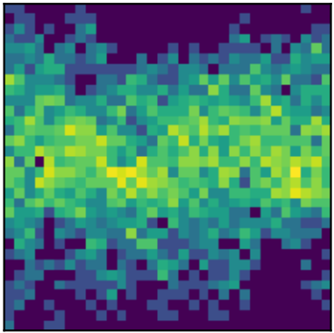
peak 26 P=1.0943d (LS)
