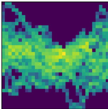
peak 47 P=9.5806d (LS)
