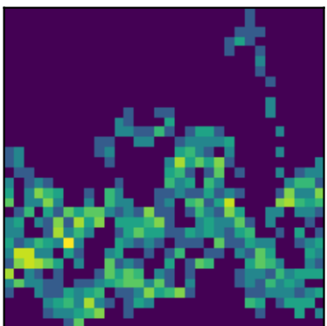
peak 14 P=0.6766d (LS)
