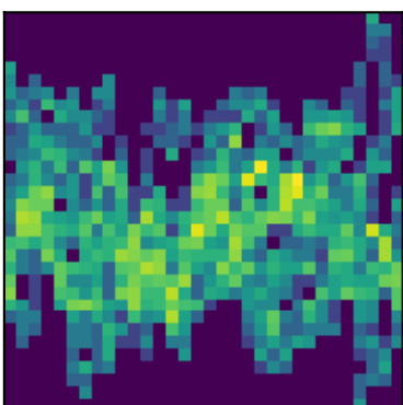
peak 33 P=0.3528d (LS)
