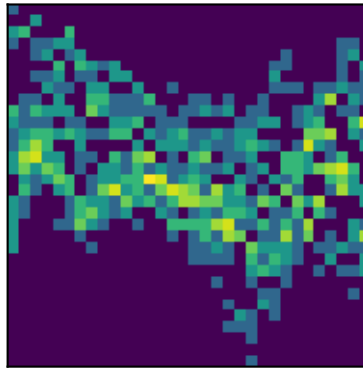
peak 11 P=1.6180d (LS)
