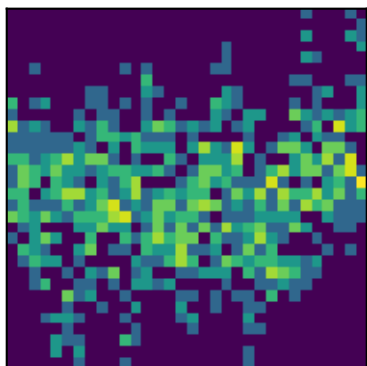
peak 14 P=0.6361d (LS)
