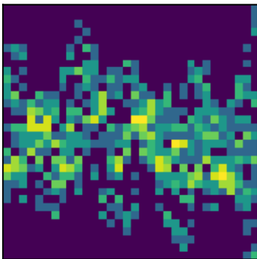
peak 12 P=0.5261d (LS)
