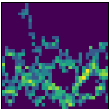
peak 15 P=0.7874d (LS)
