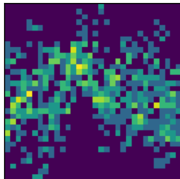
peak 12 P=0.4565d (LS)
