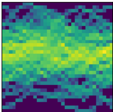
peak 18 P=1.5981d (LS)
