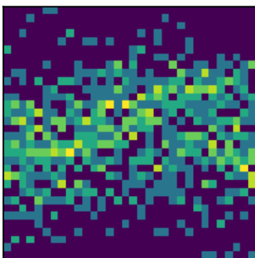
peak 8 P=2.3936d (LS)
