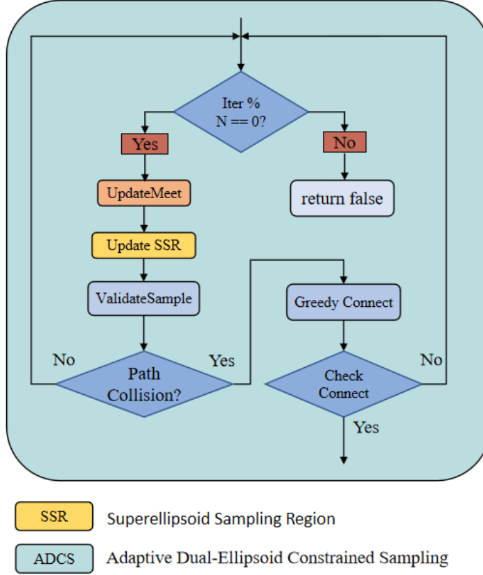
Fig. 2 Flowchart of the Adaptive Asymmetric dual-super-ellipsoid Constrained Sampling Strategy
