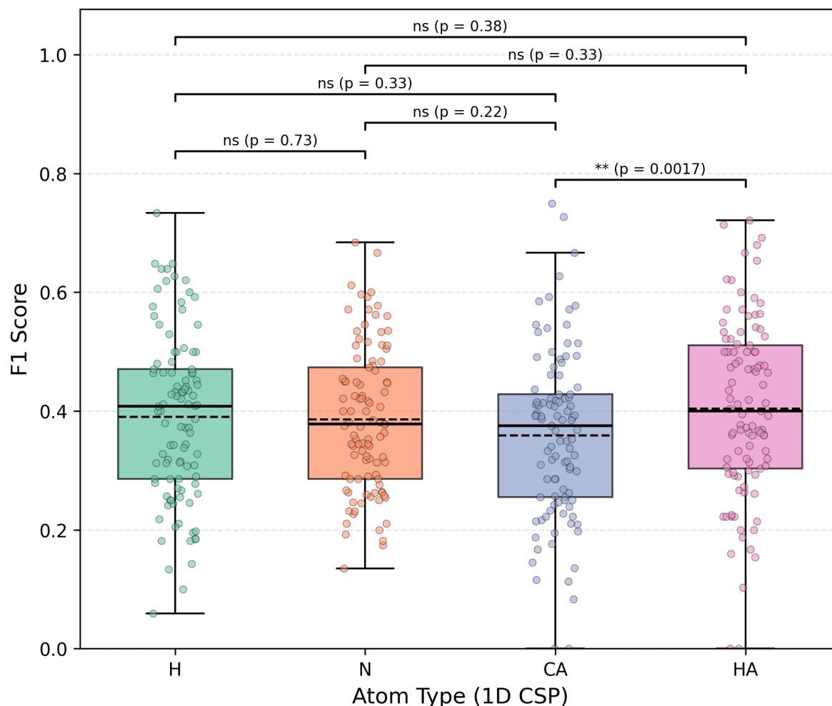
SI Fig. S15. Per-target F1 scores for 1D H/N/C \alpha /H \alpha CSPs ( n = 101 buffer-similar systems from CSP_UBQ_ph0.5_temp5C.csv with paired H/N/CA/HA F1 scores). Boxes show the per-target F1 distribution for 1D CSPs of each nucleus. Pairwise comparisons are two-sided Wilcoxon signed-rank tests for all unordered atom pairs, with Holm–Bonferroni adjustment of p -values. After Holm–Bonferroni adjustment, H, N, and C \alpha F1 scores do not differ (all adjusted p > 0.05 ). C \alpha versus H \alpha is the exception (Holm-adjusted p = 0.0017 ): median per-target F1 is 0.38 for C \alpha and 0.40 for H \alpha . Distal CSPs still occur for every nucleus at a similar frequency. Apo/holo offsets for 1D CSPs are chosen independently for each nucleus by a 1D grid search on unreferenced shifts, using the same bounds as the joint searches ( ^1\text{H}_\text{N} \pm 0.2 ppm, step 0.01 ppm; ^{15}\text{N} \pm 1.5 ppm, step 0.05 ppm; ^{13}\text{C}_\alpha \pm 2 ppm, step 0.05 ppm; ^1\text{H}_\alpha \pm 0.12 ppm, step 0.01 ppm). The CSPs calculated to retrieve an F1 score per target are calculated as (\text{dd}\langle\text{Shift}\rangle^2)^{1/2} and the threshold for significance is set as the max of the cleaned mean and 0.05 ppm, for all 1D CSPs shown in this figure.
