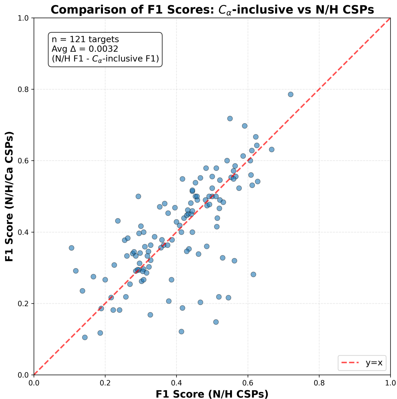
SI Fig. S12. F1 for Eqn. 1 CSPs vs Eqn. 2 CSPs ( n = 121 buffer-similar systems from CSP_UBQ_ph0.5_temp5C.csv with CA row coverage > 50\% ). F1 scores on the y axis use SI Equation S2 (combined HN+ C_\alpha ); F1 scores on the x axis use SI Equation S1 (combined HN). The F1 scores here demonstrate that per-target there are very few differences in the distribution of CSPs distant from the binding site across the n = 121 subset of targets with CA CSPs and similar experimental conditions.
