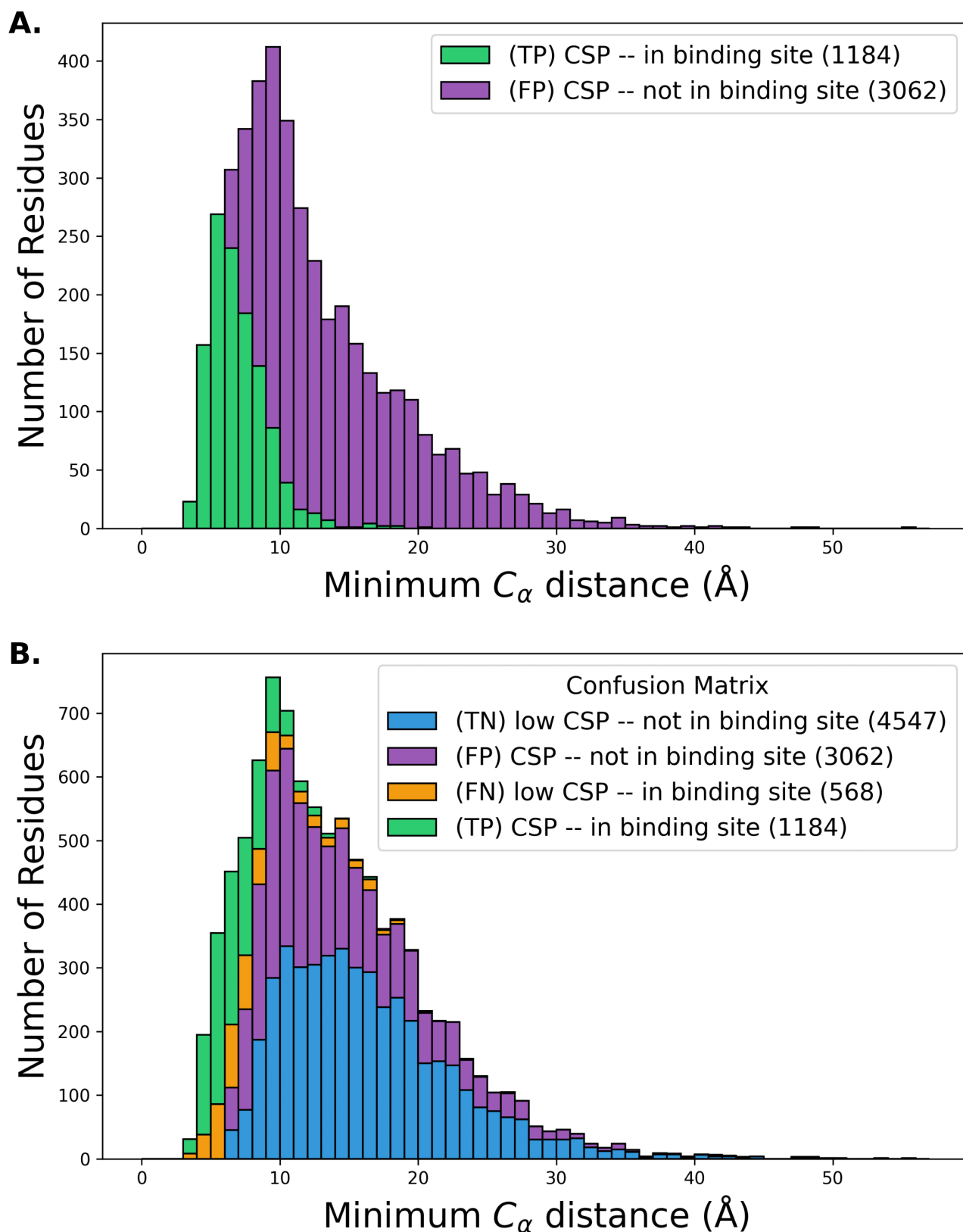
SI Fig. S11. Confusion histograms calculated with Eqn. 3 for the buffer-similar systems from CSP_UBQ_ph0.5_temp5C.csv that also have H \alpha and C \alpha shifts in both apo and holo experiments ( n = 101 ). These results are very similar to CSPs calculated using SI Equation S1. 72.2% of CSPs using SI Equation S3 are distant from the binding site compared to 69.4% using SI Equation S1.
