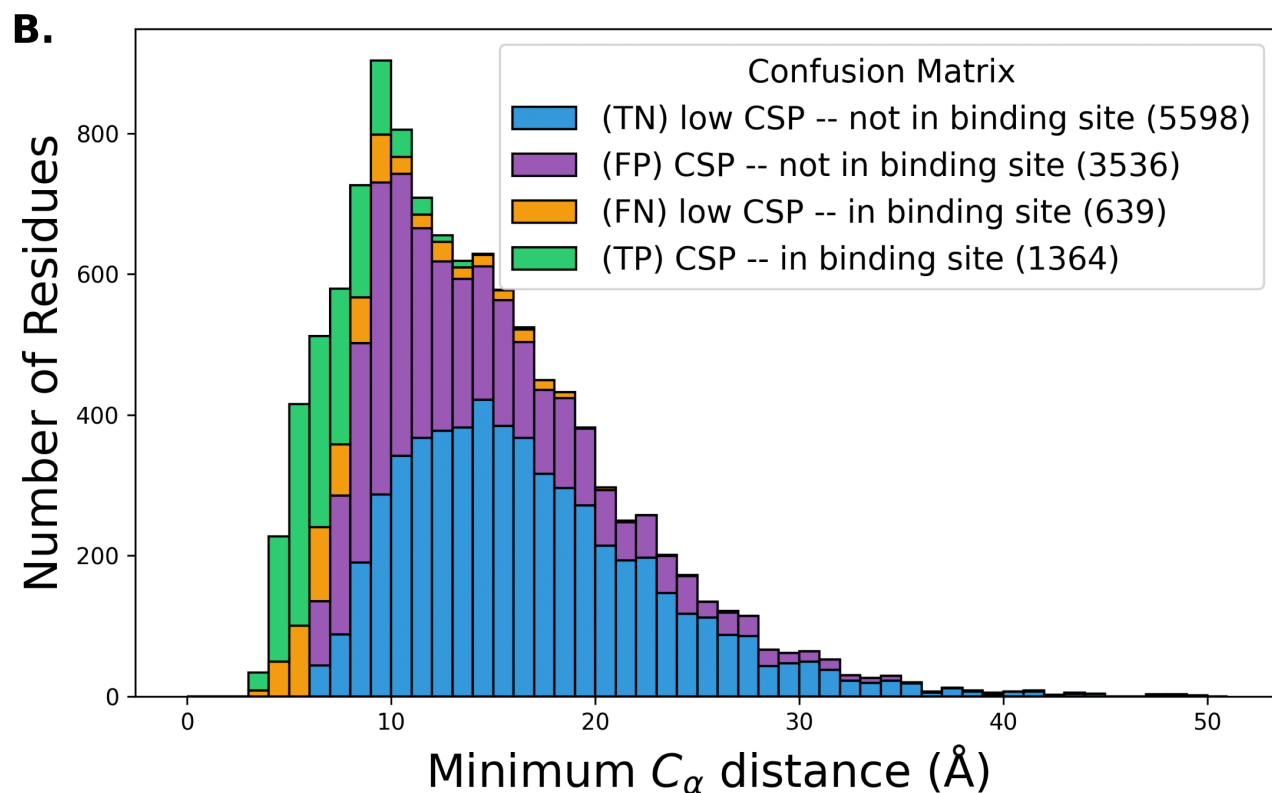
SI Fig. S10. Confusion histograms calculated with Eqn. 2 for the n = 121 buffer-similar systems from CSP_UBQ_ph0.5_temp5C.csv with CA row coverage > 50\% . These results are very similar to CSPs calculated using SI Equation S1. 72.2% of CSPs using SI Equation S2 are distant from the binding site compared to 69.4% using SI Equation S1.
