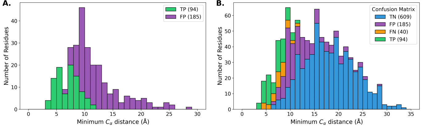
SI Fig. S7. Confusion Matrix Histograms for TFIIH Domain Receptors ( n = 9 )
