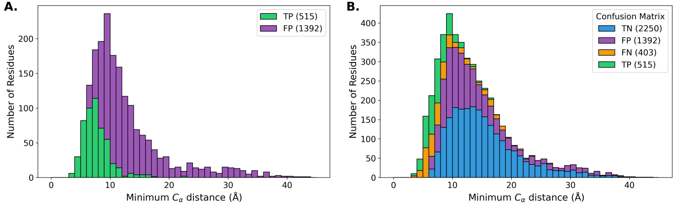
SI Fig. S3. Confusion Matrix Histograms for All Alpha Receptors
